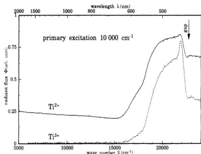
FIG. 10. Sensitization spectra of the {}^2T_2(D) \rightarrow {}^2E(D) emission of \text{Ti}^{3+}(d^1) (dashed curve) and of the {}^3T_2(F) \rightarrow {}^3A_2(F) transition of \text{Ti}^{2+}(d^2) (solid curve). Primary modulated excitation \bar{\nu} = 9800\text{--}10\,200\text{ cm}^{-1} . Detection ranges: \bar{\nu} = 3800\text{--}4800\text{ cm}^{-1} ( \text{Ti}^{3+} ), \bar{\nu} = 3100\text{--}3300\text{ cm}^{-1} ( \text{Ti}^{2+} ). T = 4.2\text{ K} .
