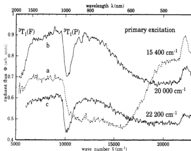
FIG. 11. Sensitization spectra of the {}^2T_2(D) \rightarrow {}^2E(D) emission of \text{Ti}^{3+}(d^1) . Primary modulated excitations: (a) 15\,050\text{--}15\,750\text{ cm}^{-1} , (b) \bar{\nu} = 19\,300\text{--}20\,700\text{ cm}^{-1} , (c) \bar{\nu} = 21\,400\text{--}23\,100\text{ cm}^{-1} . Detection range: \bar{\nu} = 3800\text{--}4800\text{ cm}^{-1} . T = 4.2\text{ K} .
