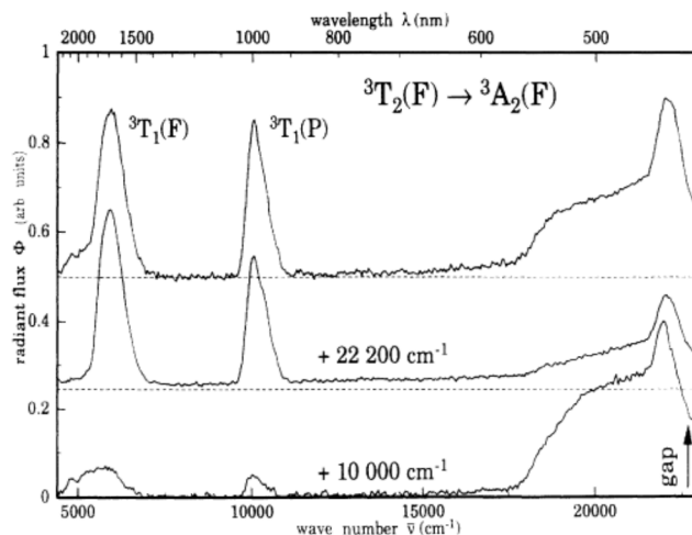
FIG. 7. Excitation spectra of the {}^3T_2(F) \rightarrow {}^3A_2(F) luminescence of \text{Ti}^{2+}(d^2) (upper curve). Detected emission range: \bar{\nu}=3100\text{--}3300\text{ cm}^{-1} . Additional unmodulated radiations: \bar{\nu}=21\,400\text{--}23\,100\text{ cm}^{-1} (middle curve), \bar{\nu}=9800\text{--}10\,200\text{ cm}^{-1} (lower curve). T=4.2\text{ K} .
