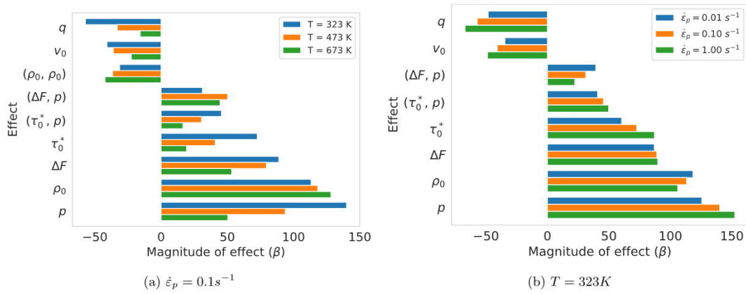
Fig. 6. The main effects and interactions effects for the yield stress (a) for \dot{\epsilon} = 0.1 s^{-1} at varying temperatures, (b) for T = 323 K at varying strain rates. The effects are in MPa, and their magnitudes are calculated using Eq. (A.3). For the definition of the material parameters see Table 2.
