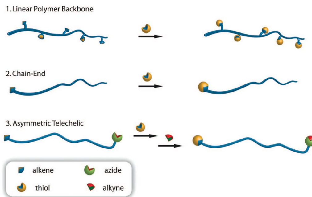
Figure 2.1.6. Schematic representation of polymer functionalization reactions examined using thiol-ene click chemistry. Reprinted with permission from Macromolecules 2008, 41, 19, 7063–7070. Copyright 2008 American Chemical Society. 14
