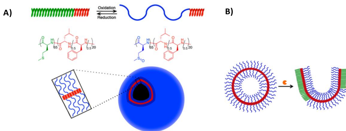
Figure 2.1.10. A) Schematic showing structure, redox properties, and proposed self-assembly of copolypeptides poly(L-methionine) 65 -b-poly-(L-leucine 0.5 -stat-L-phenylalanine 0.5 ) 20 into vesicles. B) Schematic showing a possible effect of enzymatic reduction of vesicle surface methionine sulfoxide derivative segments to methionine (sulfide) segments. Reprinted (adapted) with permission from Biomacromolecules 2013, 14, 10, 3610–3614. Copyright 2013 American Chemical Society. 61
