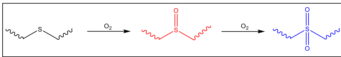
Figure 2.1.8. Oxidation reaction of polysulfides with the formation of the partially oxidized polysulfoxides, followed by its conversion into polysulfones.
