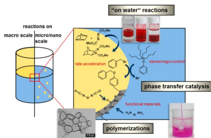
Figure 2.2.6. Schematic representation of reactions at the liquid-liquid interface. Reprinted with the permission from Chem. Rev. 2016, 116, 4, 2141–2169. Copyright 2016 American Chemical Society. 90
