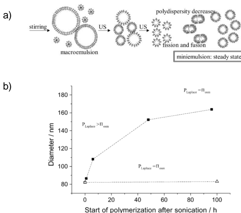
Figure 2.2.3. a) Scheme for the formation of miniemulsion by ultrasonication and b) growth of miniemulsion droplets after steady state ultrasonication with and without osmotic pressure agent. Adapted from Progress in Polymer Science, 27, Markus Antonietti and Katharina Landfester, Polyreactions in miniemulsions, 689-757. Copyright (2002), with permission from Elsevier. 69
