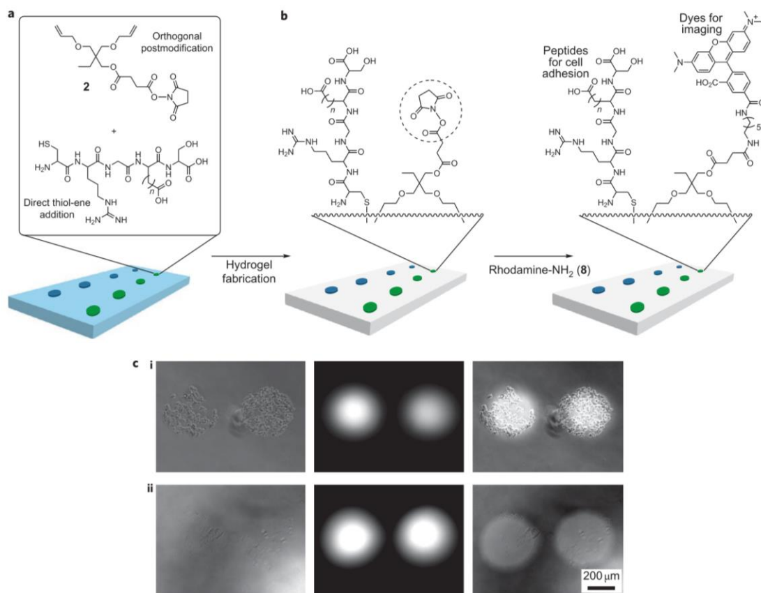
Figure 2.1.2. Combination of direct printing of peptides with orthogonal post-functionalization on individual microarray spots. a) microarray fabrication: Thiol-functional peptides (CRGDS and CRGES) and the heterobifunctional NHS cross-linker 2 were printed from a single solution and b) transferred to the hydrogel as a microarray. The activated esters were coupled with an amino-rhodamine dye ( 8 ), and these arrays were seeded with fibroblast cells. c) Microscopy images shown are of the printed cell adhesive CRGDS (i) and non-adhesive control CRGES (ii), in combination with the dye. Bright field images (left column), fluorescence images (center column) and overlay of brightfield and fluorescence images (right column). Cell growth and fluorescence are in the same area. Reprinted by permission from Springer Nature: Nature Chemistry, a versatile approach to high-throughput microarrays using thiol-ene chemistry, Gupta, N., Lin, B., Campos, L. et al. Copyright 2009. 20
