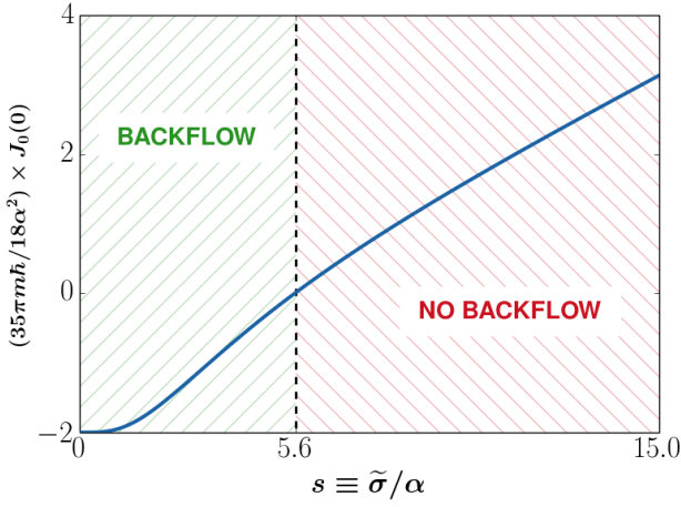
Figure 1: Scaled effective backflow current (solid blue curve), as given by (24), as a function of the (dimensionless) width s of the Gaussian precision function.
