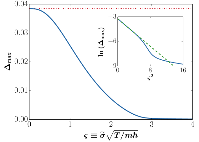
Figure 2: Behavior of the maximal eigenvalue \Delta_{\max} (solid blue curve) of the eigenvalue equation (36) with respect to the (dimensionless) width \zeta of the Gaussian precision function. The dash-dotted horizontal red line represents the Bracken-Melloy bound (15). Inset: Logarithm of \Delta_{\max} as a function of \zeta^2 (solid blue curve). The dashed green curve shows a Gaussian decay.
