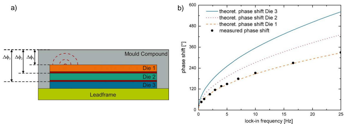
Fig. 9. (a) Cross section through a stacked IC, (b) simulated (theoretical) phase shift for a defect lying in different dies of the IC and measured phase shift values for different lock-in frequencies.
