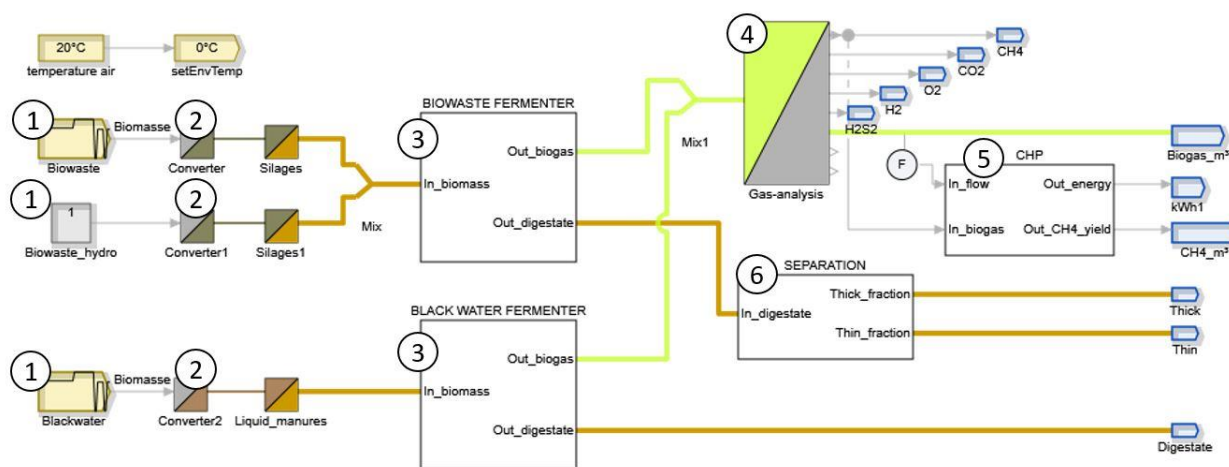
Figure 2. Simba model for in-house degradation of biowaste to heat and electricity. 1. Biomass input of biogenic waste and blackwater with 70 °C pre-treatment. 2. The Converter block determines the biomass composition. 3. The Fermenter block determines the biogas and digestate output. 4. The Gas analysis determines the biogas composition. 5. The CHP block converts biogas into energy with a calorific value of 10.5 kJ/kg. 6. The Separation block determines thick (solid) and thin (liquid) fractions.
