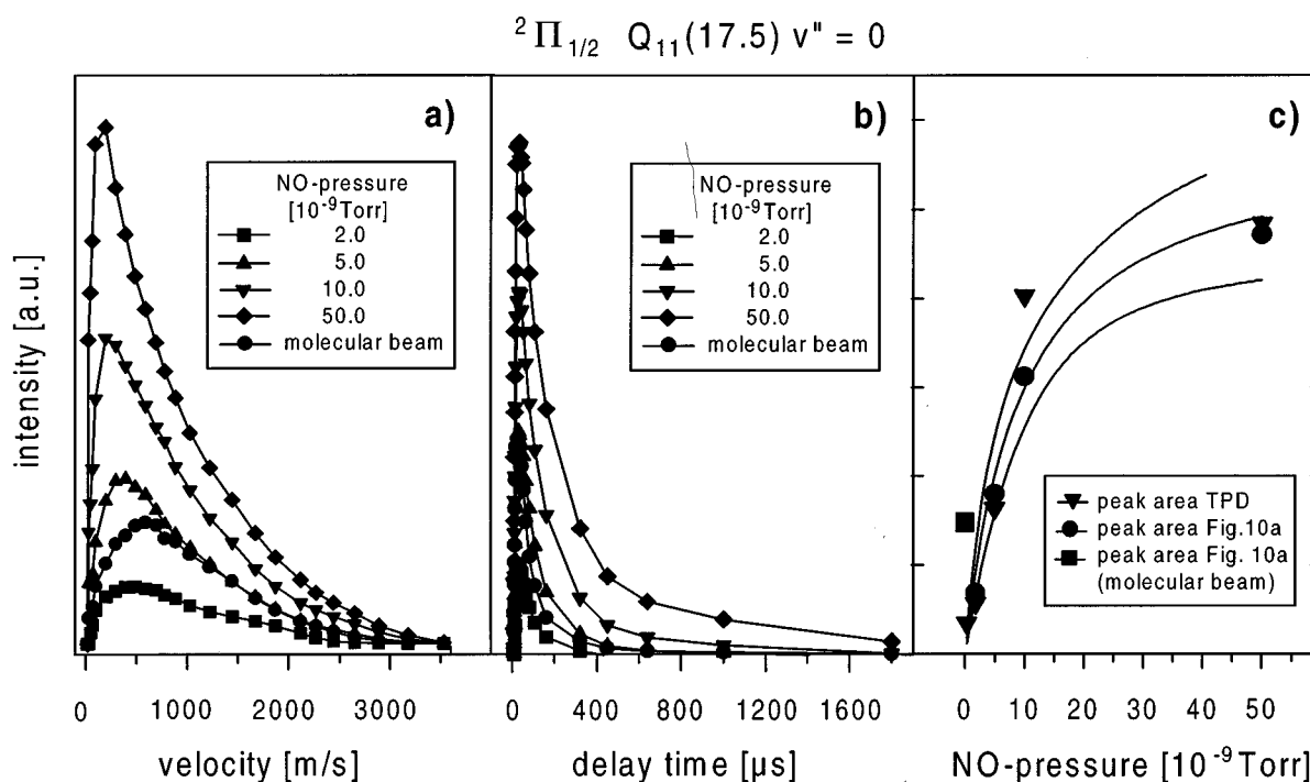
FIG. 10. (a) Velocity distributions as a function of background dosing pressure ( J''=17.5 , v''=0 , ^2\Pi_{1/2} ) of NO desorbing from \text{Cr}_2\text{O}_3(0001) after LID with 6.4 eV, filled dots: molecular beam dosing (dosing at 4 Hz, driver pulse width 700 \mu\text{s} , NO stagnation pressure=2.0 bar, nozzle diameter=800 \mu\text{m} ). (b) Corresponding original spectra as a function of time delay between desorption and detection event of (a). (c) Black dots: integrals of velocity distributions from (a) as a function of background dosing pressure. Black square: integral of velocity distribution from (a) of molecular beam dosing. Triangles: integrals of TPD spectra corresponding to velocity distributions from (a).
