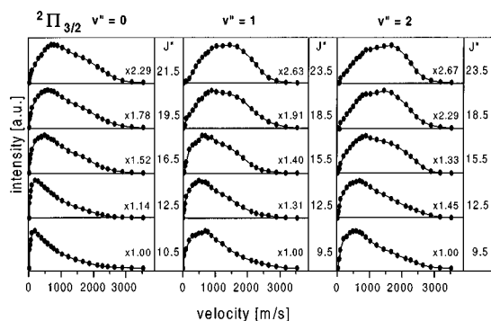
FIG. 8. Velocity distributions of NO desorbing from \text{Cr}_2\text{O}_3(0001) after LID with 6.4 eV as a function of rotational and vibrational ( v''=0,1,2 ) excitation of the desorbing molecules in the ^2\Pi_{3/2} state (maxima normalized to 1).
