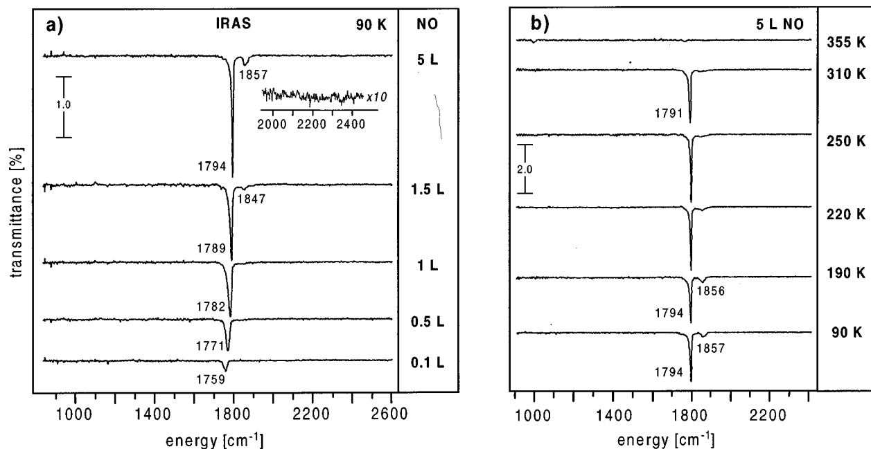
FIG. 3. (a) FTIR spectra of NO/Cr 2 O 3 (0001) as a function of coverage (dosing via needle doser). (b) FTIR spectra of NO/Cr 2 O 3 (0001) for a high coverage (dosing via needle doser) after subsequent short heating to different temperatures.
