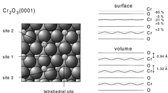
FIG. 1. Schematic drawing of the \text{Cr}_2\text{O}_3(0001) surface.
