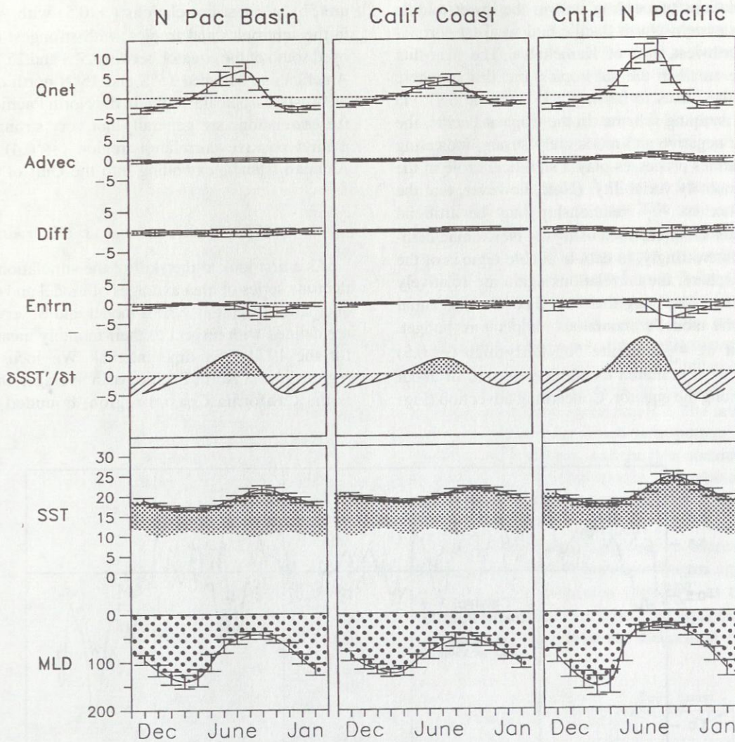
FIGURE 4 Long-term mean and standard deviation of model heat budget terms \frac{\Delta SST}{\Delta t} , SST ( ^{\circ}\text{C} ), and mixed layer depth (m) for the North Pacific basin, the California Coast, and the central North Pacific regions. Units are 0.1^{\circ}\text{C mo}^{-1} for heat-budget terms and \frac{\Delta SST}{\Delta t} .
