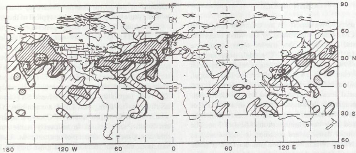
FIGURE 2 Correlation coefficients ( \times 100 ), mapped for global ocean Q'_{l+s} vs. \frac{\Delta SST}{\Delta t} at each grid point, for the winter months, 1946-1986. Contours at 0.3, 0.5, and 0.7. Light and heavy shadings indicate correlations \geq 0.3 and \geq 0.5 .
