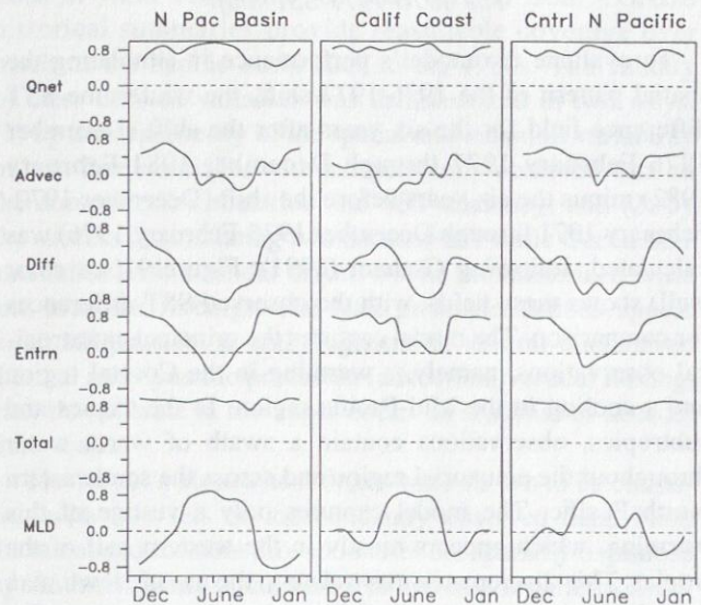
FIGURE 8 Correlation between \frac{\Delta SST'}{\Delta t} and: each of the anomalous model heat-budget forcing terms (right-hand side of Equation 4); their total; and anomalous MLD for the North Pacific basin, California Coastal, and central North Pacific regions. Stratified by month, from 1970-1988.
