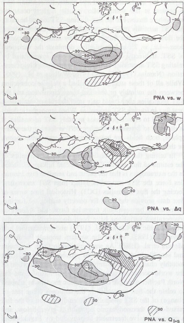
FIGURE 1 The correlation coefficients ( \times 100 ) between time series of the amplitudes of Pacific-North American EOF and our all-grid-point time series of w' (above), \Delta q' (middle), and Q'_{l+s} (below) in the North Pacific for the winter months, 1950-1986. Solid contours show PNA pattern. Significant correlation regions are superimposed upon the EOF patterns; shading indicates regions where the magnitude of the correlation is \geq 0.3 . Significant positive/negative correlations are shown by stippling, hatching in upper two frames; and by hatching, stippling in lower frame.
