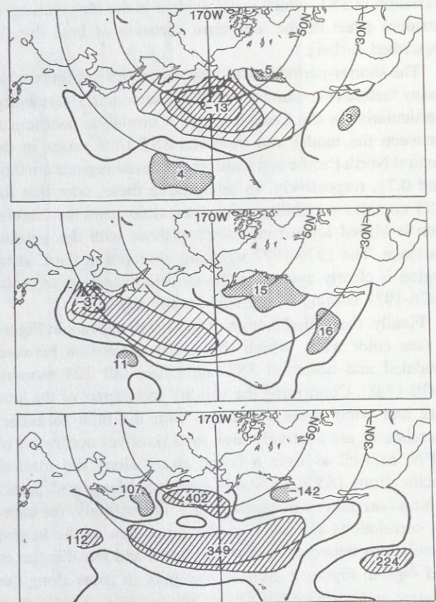
FIGURE 10 Difference fields of observed winter SLP (mb; top), heat flux ( \text{W m}^{-2} ; middle), and \{w^3\} , the pseudo-total kinetic energy ( \text{m}^3 \text{s}^{-3} ; bottom), for the winters of 1976-77 through 1981-82 minus those of 1970-71 through 1975-76.
