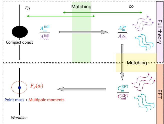
FIG. 1. Schematic calculational process to determine the response function F_\ell(\omega) . The response is defined in an effective description (EFT) where the compact object is viewed from large distances and appears as a point mass with multipole moments. Grey arrows indicate the information flow from the microphysical properties of the object to the response via the ratio of in- and outgoing wave amplitudes at infinity. In the full theory calculations based on relativistic perturbations, we specialize to a black hole, thus need only the solutions in the exterior of the horizon r_H , and base the matching of the near-horizon and asymptotic solutions on analytical approximations for M\omega \ll 1 . The matching to the effective theory is achieved by identifying in- and outgoing wave states at null infinity.
