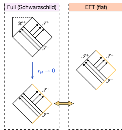
FIG. 2. Penrose diagrams illustrating the asymptotic identification of null infinities ( \mathcal{I}^\pm ) of the Schwarzschild spacetime in the limit that the size of the black hole r_H shrinks to zero and the Minkowski spacetime we use in the effective description. The matching is performed using double null coordinates adapted to the lightcones.
