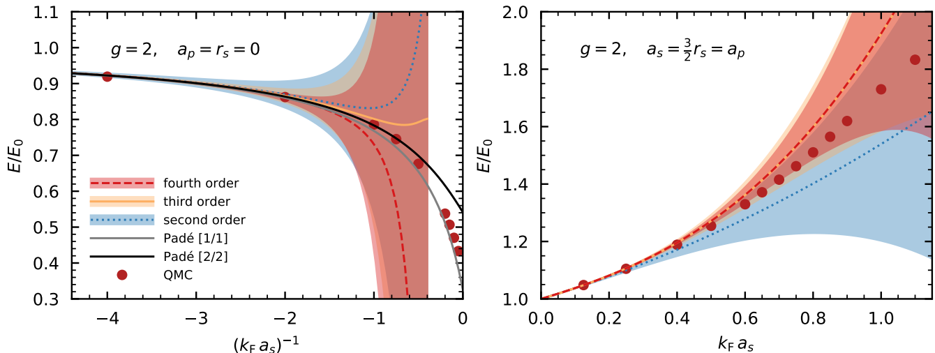
Figure 4. Convergence behavior of the Fermi-momentum expansion for the ground-state energy E/E_0 of a dilute Fermi gas of spin one-half fermions with a_p = r_s = 0 (LO, left panel) and a_s = 3r_s/2 = a_p (HS, right panel) at negative and positive k_F a_s , respectively. The respective uncertainty bands correspond to the 68% credibility intervals from our Bayesian estimation of the next-higher coefficient in the k_F a_s expansion. In the LO case we also show results obtained from two different Padé approximants, Padé[1, 1] (gray line) and Padé[2, 2] (black line). Finally, the thick red dots in each panel correspond to results from nonperturbative QMC computations [8, 64, 65]. Note that the x -axes in the two panels are different, and based on the available QMC data we show the attractive regime with a_s < 0 in the left panel and the repulsive regime with a_s > 0 in right panel. See the text for more details.
