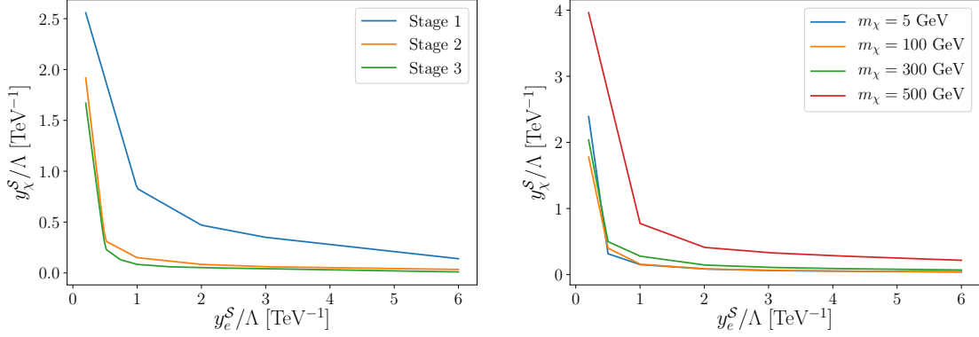
Figure 4.20: Left panel: Comparison of the expected limits on the couplings obtained at the three stages of CLIC, assuming m_S = 200 GeV and m_\chi = 5 GeV.
