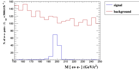
Figure 4.19: Comparison of signal and background shape in m_{ee} for CLIC stage III. The signal corresponds to y_e^S/\Lambda = 1.5/\text{TeV} and y_\chi^S/\Lambda = 0.25/\text{TeV} , close to the later derived exclusion limit.
