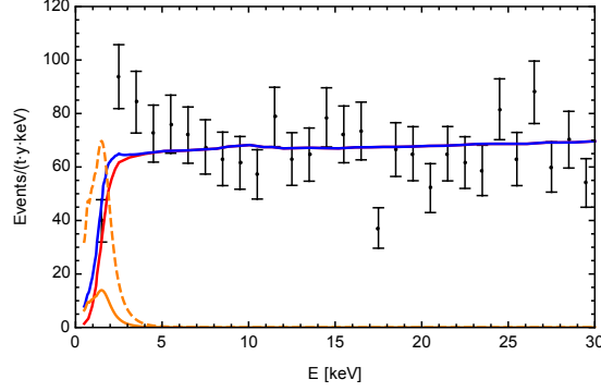
Figure 4.23: Comparison between the best fit differential event rate for a DM particle with m_\chi = 10 GeV and \sigma_{e\chi} = 1.25 \times 10^{-39} cm 2 and the data. The style is similar to Fig. 4.22, and for better visualization we also show the signal rate enhanced by a factor of 5 as an orange dashed line.
