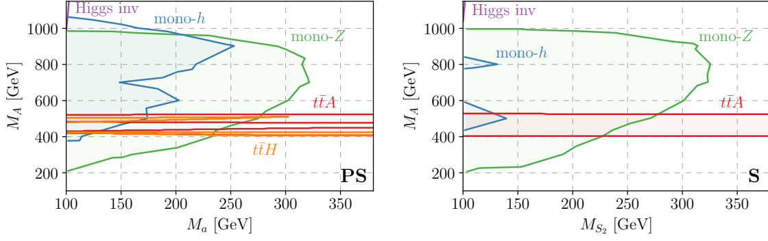
Figure 2.13: Overview of the 2\sigma exclusion limits from searches for mono- h , mono- Z , t\bar{t} resonances and Higgs-to-invisible in the M_{a/S_2} - M_A plane for the 2HDM+PS (left) and 2HDM+S (right); see text for details. In both plots we use the parameters given in Eq. (2.43) and set \tan\beta = 1 . Limits from ID and DD vanish for an appropriate choice of m_\chi .
