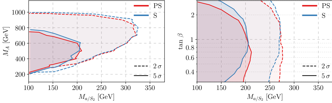
Figure 2.9: 2\sigma (dashed) and 5\sigma (solid) exclusion limits from mono- Z searches in the M_{a/S_2} - M_A (left) and M_{a/S_2} - \tan\beta plane (right) for the 2HDM+S (blue) and PS (red). In both plots we use the parameters as given in Eq. (2.43) with \tan\beta = 1 for the left one and M_A = 500 GeV for the right one.
