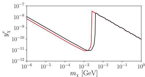
Figure 4.24: Isocontours of correct DM relic density assuming production through freeze-in and considering the assignments of model parameters for BM1 (red) and BM2 (black). The reheating temperature T_R has been set to 100 GeV.
