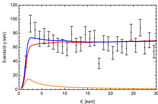
Figure 4.22: Comparison between an exemplary differential event rate for a scalar with m_s = 60 eV and \sqrt{y_e^s y_\nu^s} = 7.9 \times 10^{-7} , corresponding to the best fit point, and the observations in [330]. The full differential event rate is shown in blue, while the pure signal (background) contribution is depicted in orange (red).
