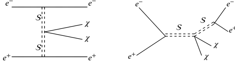
Figure 4.18: Feynman diagrams for \chi\bar{\chi} + e^+e^- production at CLIC — for the LHC case, the electrons can be replaced with up or down quarks.
