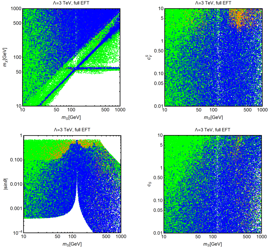
Figure 4.6: Results of the parameter scan for the scalar eDMEFT setup in the m_S – m_\chi , m_S – c_V^S , m_S – |\sin\theta| , and m_S – c_S planes. The green points provide the correct relic density according to the WIMP paradigm, while the orange points are, in addition, compatible with constraints from DD. The blue points are, finally, also compatible with collider constraints. See main text for details on the scan and the constraints accounted for.
