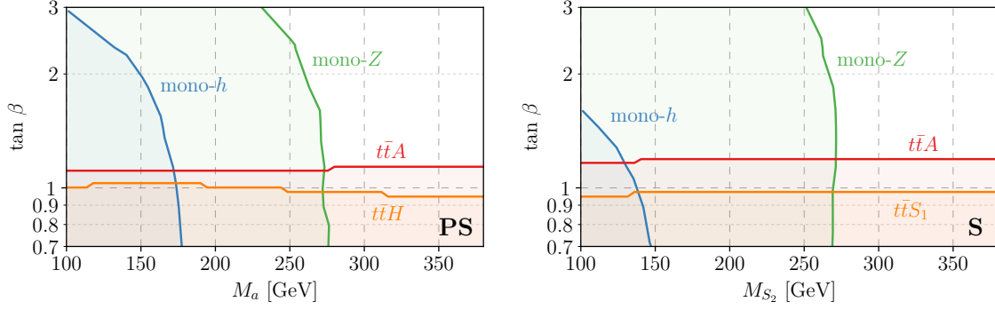
Figure 2.14: Overview on the 2\sigma exclusion limits from searches for mono- h , mono- Z , t\bar{t} resonances and Higgs-to-invisible in the M_{a/S_2} - \tan\beta plane for the 2HDM+PS (left) and 2HDM+S (right); see text for details. In both plots we use the parameters given in Eq. (2.43) and set M_A = 500 GeV. Limits from ID and DD vanish for an appropriate choice of m_\chi .
