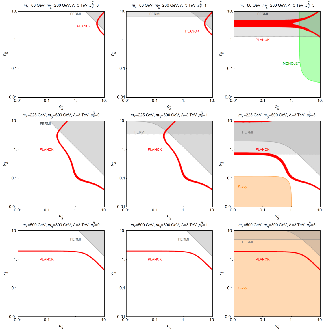
Figure 4.14: Summary of constraints in the c_{\bar{S}}-y_{\bar{S}} plane for c_V^{\bar{S}} = 0 (left column), c_V^{\bar{S}} = 1 (center column), and c_V^{\bar{S}} = 5 (right column) and three different mass assignments as indicated in the individual panels. The red contours correspond to the correct relic density while regions excluded by ID are depicted in dark grey for \gamma -ray continuum and in light grey for \gamma -ray line searches. Orange regions are excluded by collider searches for resonances decaying into photons and the green region by mono-jet searches.
