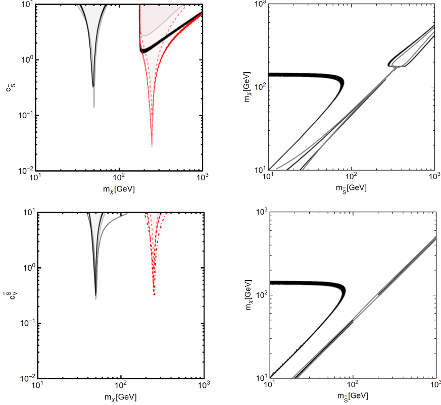
Figure 4.12: Isocontours of the correct relic density for the Yukawa (top), and gauge (bottom) portals. The left column display the m_\chi -coupling plane for m_{\tilde{S}} = 100 GeV (black) and m_{\tilde{S}} = 500 GeV (red). The shaded regions, and the regions inside the dashed lines represent bounds from ID for the corresponding BMs. The right column shows the m_{\tilde{S}}-m_\chi plane for y_{\tilde{S}} = 1 and c_{\tilde{S}} = 1 (top) and c_{\tilde{V}} = 1 (bottom). The regions inside the gray contours are excluded by ID. For all plots we set \Lambda = 3 TeV.
