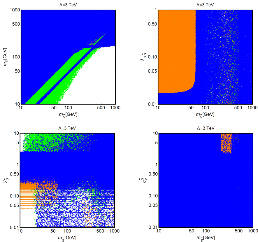
Figure 4.15: Results of the parameter scan for the pseudoscalar eDMEFT projected in the m_{\tilde{g}}-m_\chi and m_{\tilde{g}} -coupling planes, analogous to the scalar mediator case presented in Fig. 4.6 and 4.7 without the m_{\tilde{g}}-c_{\tilde{g}} plane, since the latter is not impacted by the considered constraints. Green points account only for the correct relic density, orange points are excluded by collider searches, while blue points pass all applied constraints, see text for more details.
