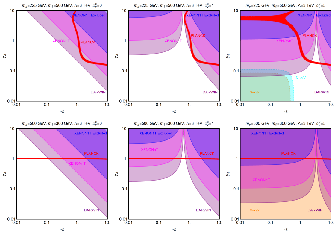
Figure 4.5: Summary of constraints in the c_S - y_S plane and setting the h - S mixing to zero for the benchmark masses from the second and third row of Fig. 4.3 with the same color code. The case m_\chi = 80 GeV, m_S = 200 GeV is not shown, since it does not allow for the correct relic density.
