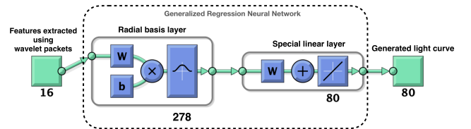
Figure 4. Shallow two-layer generalized regression neural network with Gaussian kernels used to synthesize simulated light curves from a limited amount of training data. \mathbf{W} represents the Weight, and \mathbf{b} is the bias used in the respective neural network hidden layer. The number of radial basis layers (278) equals the number of training datasets. We use 80% of light curves from 87 verified GRB events and use the data from all four quadrants.
