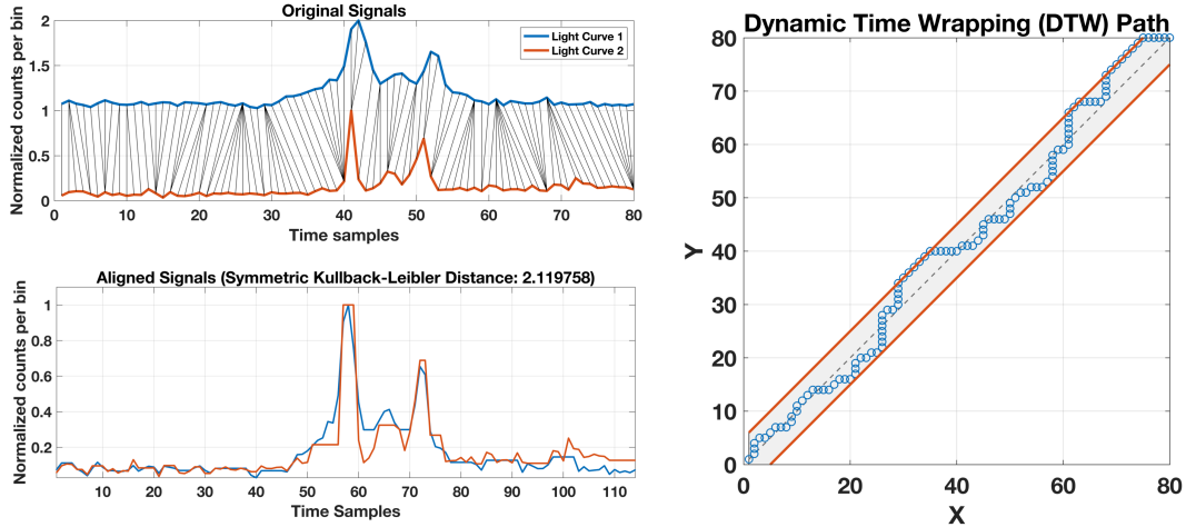
Figure 3. Distance between two GRB light curves estimated using DTW with symmetric Kullback-Leibler metric and an adjustment window size of 5 samples. Each curve is individually normalized based on its peak height.
