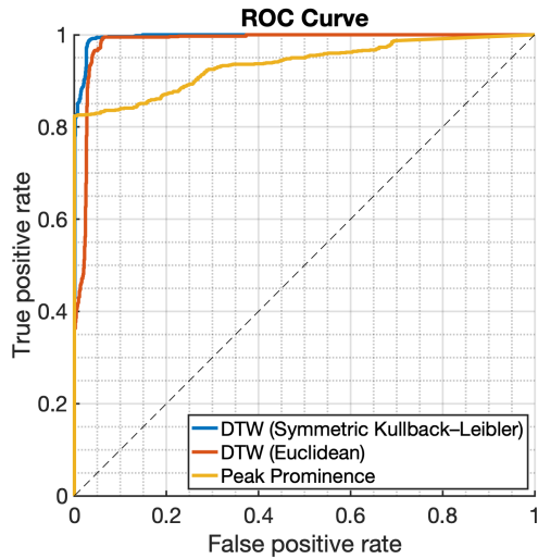
Figure 5. Receiver Operator Characteristic (ROC) curve depicting the true positive rate vs. the false positive rate for both the DTW template matching scheme and a traditional peak detection algorithm. Curves are generated by varying the respective threshold parameter, DTW distance, and the peak prominence.
