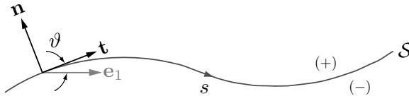
Figure 1.1 The interface \mathcal{S} . Our convention is that K be positive on concave upward portions of \mathcal{S} . The symbols (\pm) label the phases on the two sides of the interfaces.
