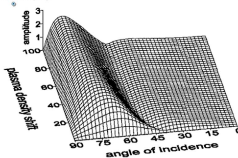
FIG. 2. Amplitude |B_+|/B_0 versus the angle of incidence \theta_0 and plasma density shift \Delta N/N_1 for \omega_{p1}/\omega_0 = 0.5 and d\omega_0/c = 2 .
