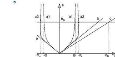
FIG. 1. Kinematic diagram in-plane wave vector h versus frequency \omega . ( a_1, a_2 ) Dispersion curves for surface waves guided by the plasma layer of plasma frequency \omega_{p2} for thick layer \omega_{p2}d/c > 0.73 and thin layer \omega_{p2}d/c < 0.73 , respectively, \omega = \omega_{p2}\sqrt{2} is the asymptotic value of frequency as h \rightarrow \infty ; ( b ) light-lines h = \omega/c ; ( c ) line h = (\omega/c)\sin\theta_0 . Frequencies of the excited surface waves \omega_{s0} are shown only for the case of thin plasma layer.
