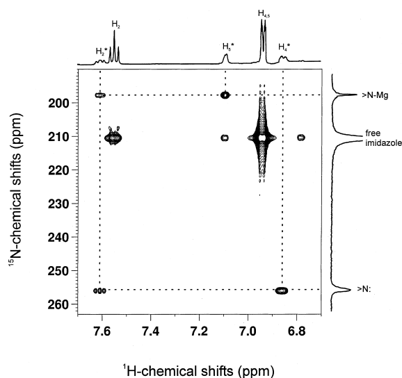
Fig. 2. 600 MHz ^{15}\text{N} - ^1\text{H} HMBC spectrum of imidazole (enriched to 95% ^{15}\text{N} at both nitrogens) complexed with BChl a in THF (10% d 8 ) at 25°C, showing the cross-peaks between proton and nitrogens of bound imidazole. * resonance of ^1\text{H} in the imidazole ring bound with BChl a .
