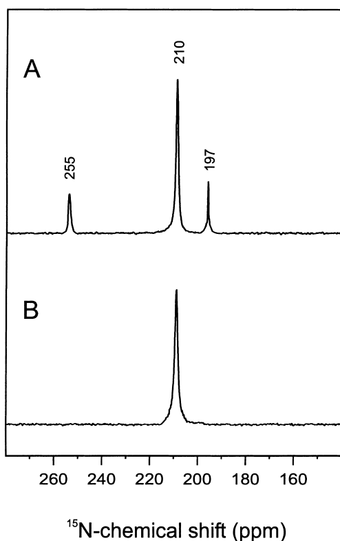
Fig. 1. The 600 MHz one-dimensional ^{15}\text{N} -NMR spectrum of imidazole (enriched to 95% ^{15}\text{N} at both nitrogens) complexed with BChl a (A) or BPheo (B) in THF (10% d_8 ) at 25°C. For the ^{15}\text{N} -NMR spectrum 5000 scans with 0.3 s repetition time were measured. The numbering system of the imidazole ring is indicated in Scheme 1.
