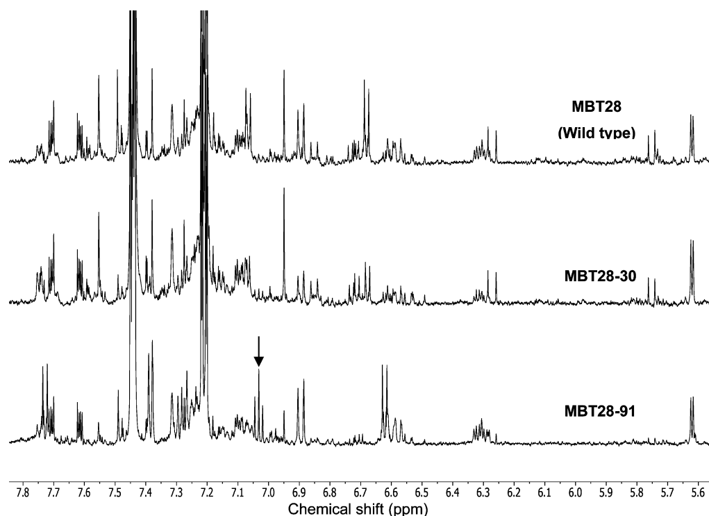
Figure 2. Comparison of ^1\text{H} NMR spectra. ^1\text{H} NMR (600 MHz) was done on samples from Streptomyces sp. MBT28 and its \text{Str}^{\text{R}} mutants MBT28-30 and MBT28-91. The solvent was \text{CH}_3\text{OH}-d_4 , and peaks are shown for the region of \delta 5.6–7.8 ppm. The signal at \delta 7.03 (t, J = 7.2 Hz) that was exclusively identified in mutant MBT28-91 is highlighted by an arrow.
