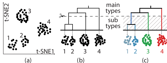
Fig. 5. Two-Level Color-Coding . Clusters from the embedding, a), are hierarchically clustered, b), and a user-defined threshold is used to define main- and sub-types. Finally, color hues are assigned to the main-types and different saturation is applied to the corresponding sub-types, c).
