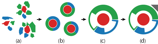
Fig. 10. Glyph Design , representing a motif of a unique microenvironment (only blue and green cells) for a red cell. a. b) each microenvironment can be abstracted as described in Fig. 9. In c), we combine the different instances of the motif to a single glyph, showing the mean frequencies and variation. Finally, in d) we add an indicator for the significance of the motif.
