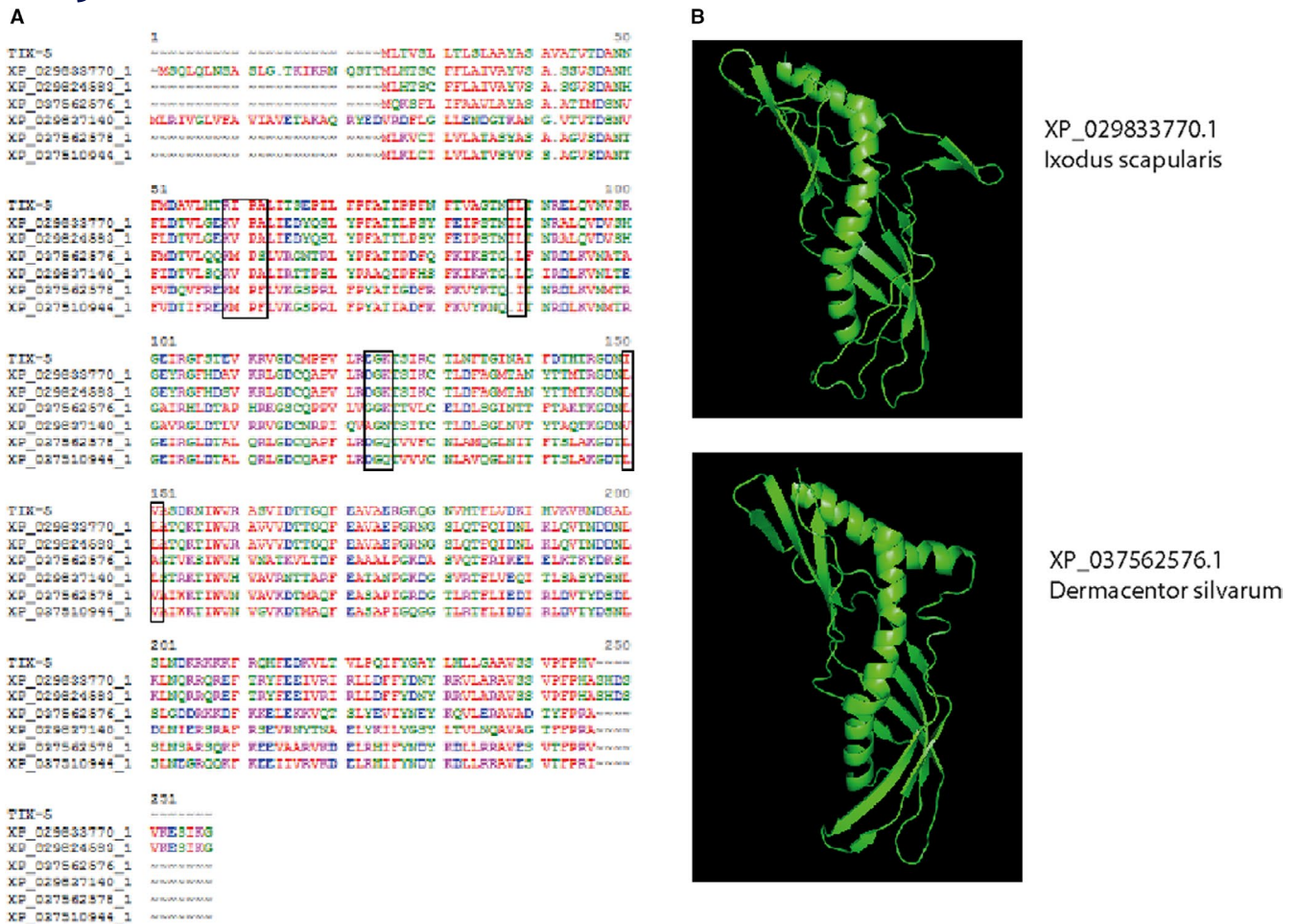
FIGURE 7 Tick inhibitor of factor Xa (TIX) toward FV homology family members. (A) The mature amino acid sequence of TIX-5 was aligned with six nearest homologues, all found in tick species. (B) Phyre2 predicted structures of XP_029833770.1 ( Ixodus scapularis ) and XP_037562576.1 ( Dermacentor silvarum ) are shown as ribbon diagram. The images in panel B were generated using Pymol software. 24
