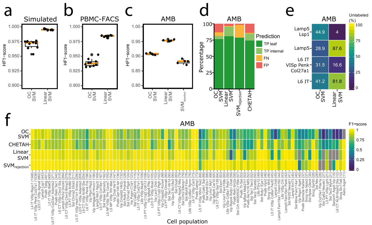
Fig. 3 Classification performance. a–c Boxplots showing the HF1-score of the one-class and linear SVM during n -fold cross-validation on the a simulated ( n = 10), b PBMC-FACS ( n = 10), and c AMB ( n = 5) dataset. In the boxplots, the middle (orange) line represents the median, the lower and upper hinge represents the first and third quartiles, and the lower and upper whiskers represent the values no further than 1.5 interquartile range away from the lower and upper hinge, respectively. d Barplot showing the percentage of true positives (TP), false negatives (FN), and false positives (FP) per classifier on the AMB dataset. For the TPs a distinction is made between correctly predicted leaf nodes and internal nodes. e Heatmap showing the percentage of unlabeled cells per classifier during the different rejection experiments. f Heatmap showing the F1-score per classifier per cell population on the AMB dataset. Gray indicates that a classifier never predicted a cell to be of that population.
