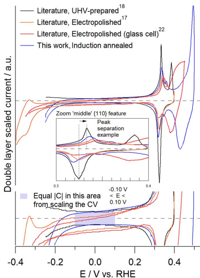
Figure 3. Comparison of literature reported CVs of Cu(110) with an induction annealing-prepared sample. CVs have been manually shifted up/down to reach the maximum amount of symmetry around the x -axis of the main adsorption features. CVs have been scaled to the absolute charge of the CV region represented by the blue dotted box, with the potential boundaries as specified in the image.
