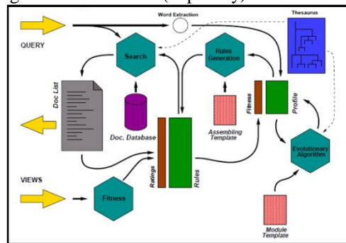
Fig 4 - Working of a Learning Search Engine based on User Profiles [5]
