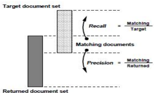
Fig 2: Recall rate and Precision rate
