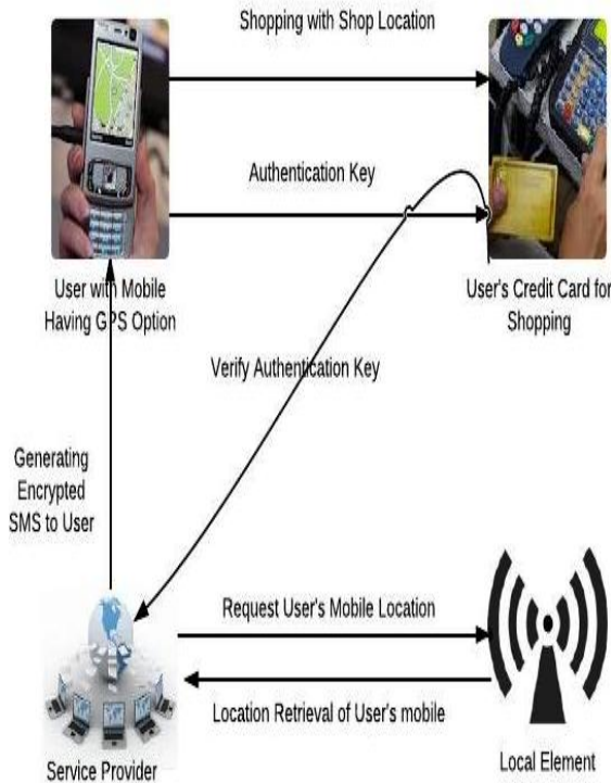
Fig.1.1 Login-Authentication Overview
