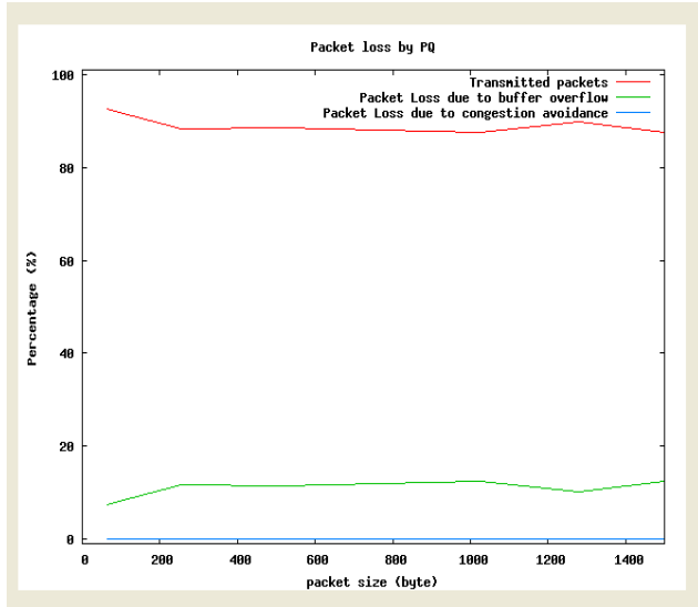
Fig 3.4. PQ Packet Loss Performanc
