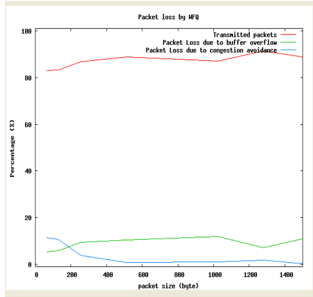
Fig 3.2. WFQ Packet Loss Performance
