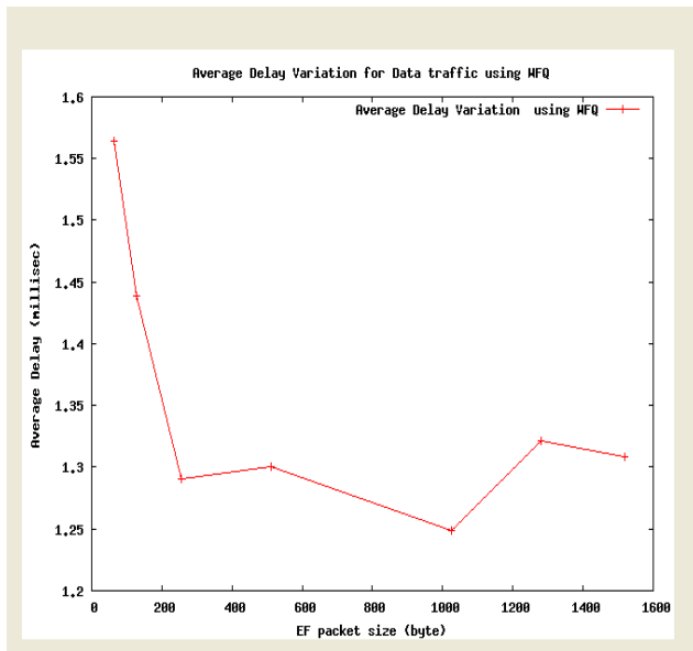
Fig 3.1. WFQ Average Delay Performance
