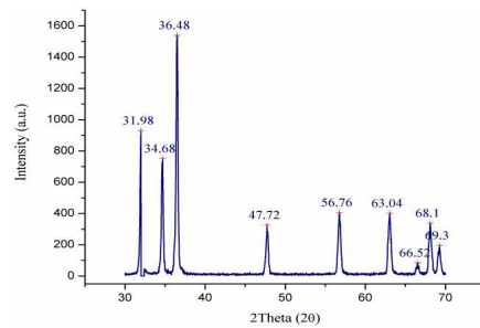
Figure 8 XRD data obtained from ZnO samples. The peaks are similar to the characteristic peaks of the wurtzite structure.8
