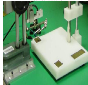
Fig 5 closer view of fotonic displacement sensor probe and PVDF electrospun specimen.
