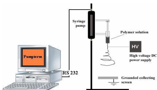
Figure 1 Schematic representation of the computer controlled electrospinning setup. Up to 100 syringe pumps can be independently controlled via one unit.
