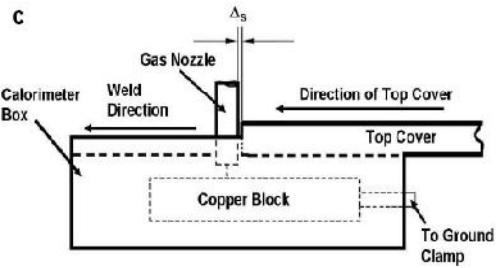
Fig. 2 (a) Dimensions of the groove; (b) calorimeter design showing the inside of the insulated box with the copper block; and (c) schematic showing how the calorimeter works while welding.
