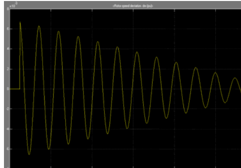
Fig.10.Rotor speed deviation
