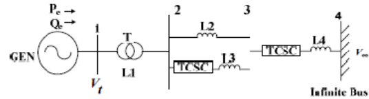
Fig. 3 : Single machine infinite-bus
