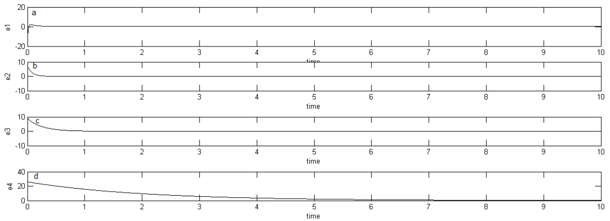
Fig. 4. Dynamics of anti-synchronization errors for two identical hyperchaotic Chen systems (master system (2) and slave system (3)) (a) e_1 ; (b) e_2 ; (c) e_3 ; (d) e_4 .
