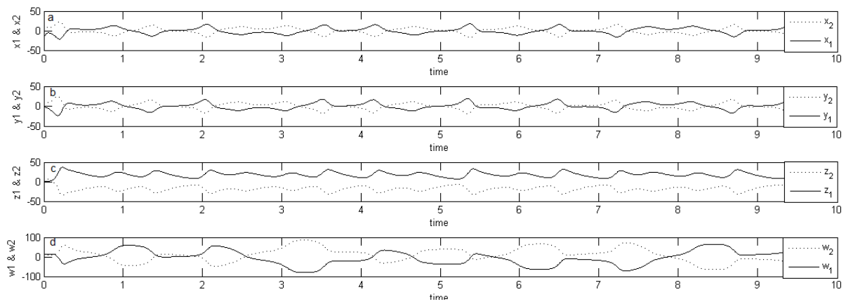
Fig. 3. The time response of states for master system (2) and the slave system (3) for anti-synchronization via active backstepping (a) signals x_1 and x_2 ; (b) signals y_1 and y_2 ; (c) signals z_1 and z_2 ; (d) signals w_1 and w_2 .
