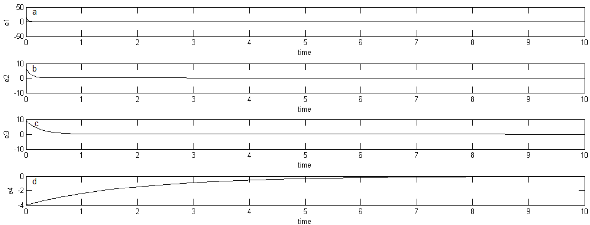
Fig. 2. Dynamics of synchronization errors for two identical hyperchaotic Chen systems (master system (2) and slave system (3)) (a) e_1 ; (b) e_2 ; (c) e_3 ; (d) e_4 .
