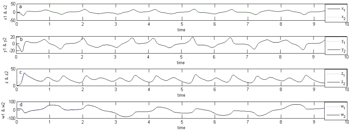
Fig. 1. The time response of states for master system (2) and the slave system (3) for synchronization via active backstepping (a) signals x_1 and x_2 ; (b) signals y_1 and y_2 ; (c) signals z_1 and z_2 ; (d) signals w_1 and w_2 .
