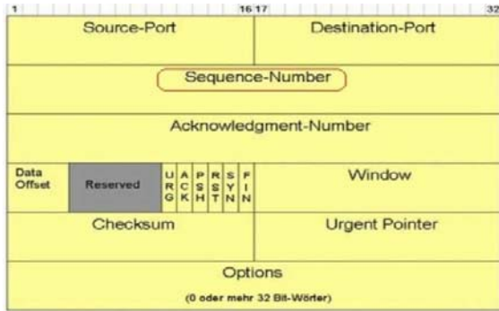
Figure 5: TCPv4 header
