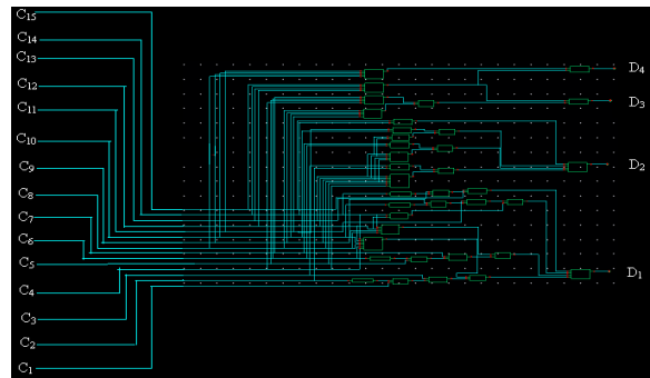
Fig. 4: Priority encoder stage
