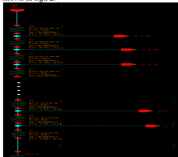
Fig. 2: Resistor string for proposed flash ADC.
