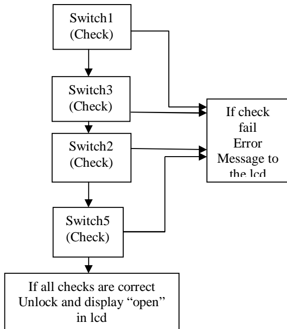
Fig2 Algorithm Explanation
