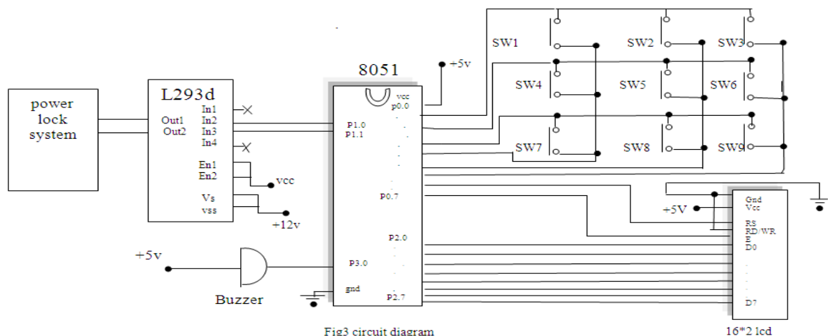
Fig3 circuit diagram
