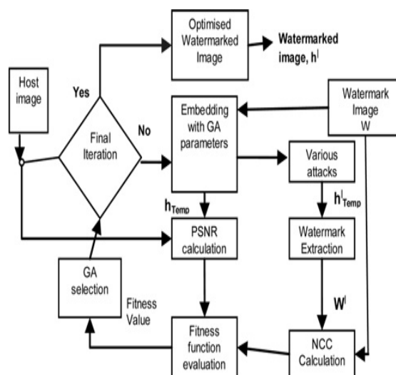
Figure 4 Genetic Algorithm based Watermark Insertion
