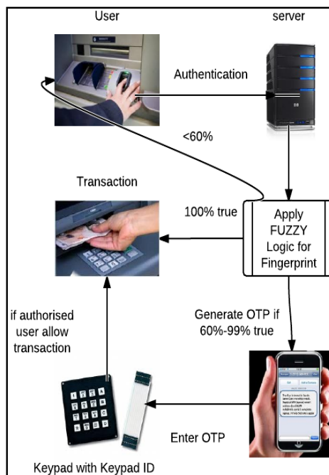
Fig.1.2 Login-Authentication Overview
