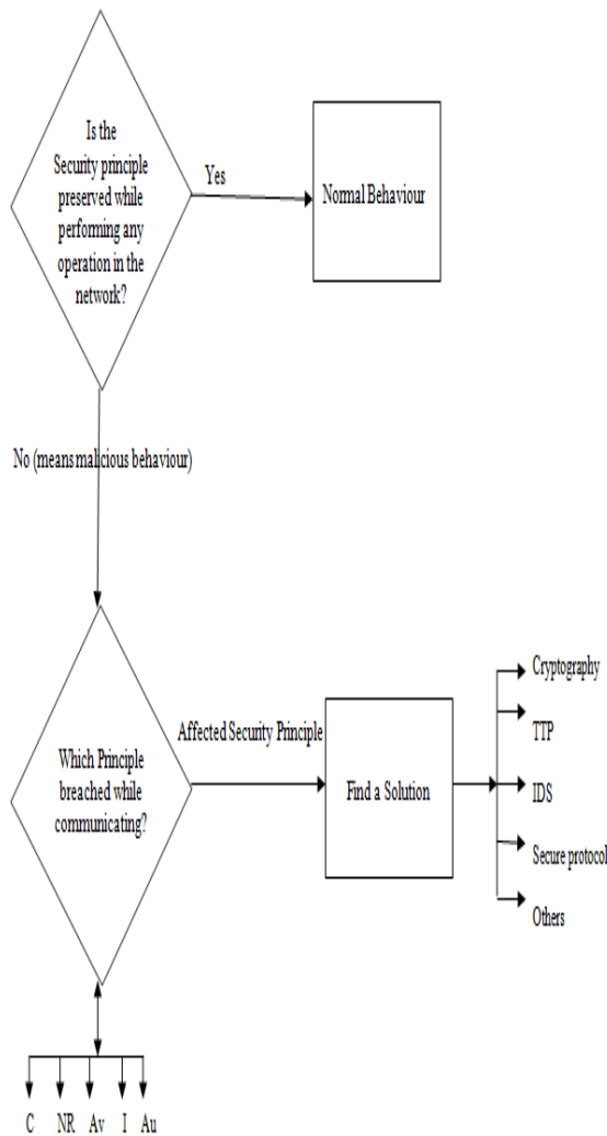
Defined Algorithm for Normal and Malicious behavior of a node
