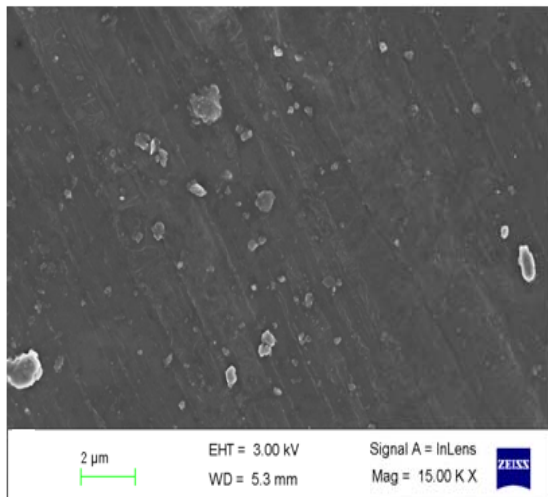
Figure 7b. SEM of Alumina modified PP/HDPE/EVA/PLA (80/20/5/4) blend.
