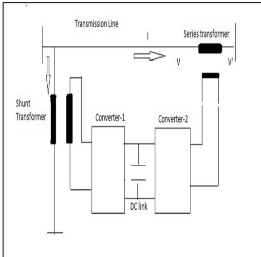
Fig.3. Schematic diagram of UPFC.
