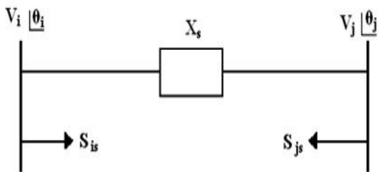
Fig.6. Injection model for a series connected VSC. Shunt connected voltage source converter model:
