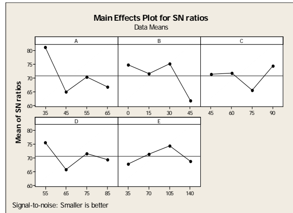
Figure 3. Effect of control factors on erosion rate for hybrid composites
