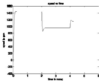
Fig2. Rotor Speed
