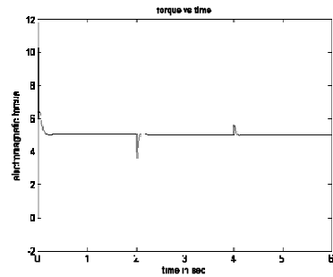
Fig5.Electromagnetic Torque
