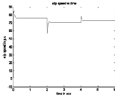
Fig4.Slip Speed
