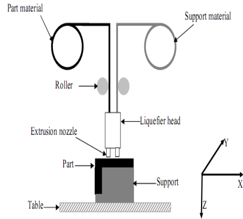
Fig. 2 Schematic description of FDM process
