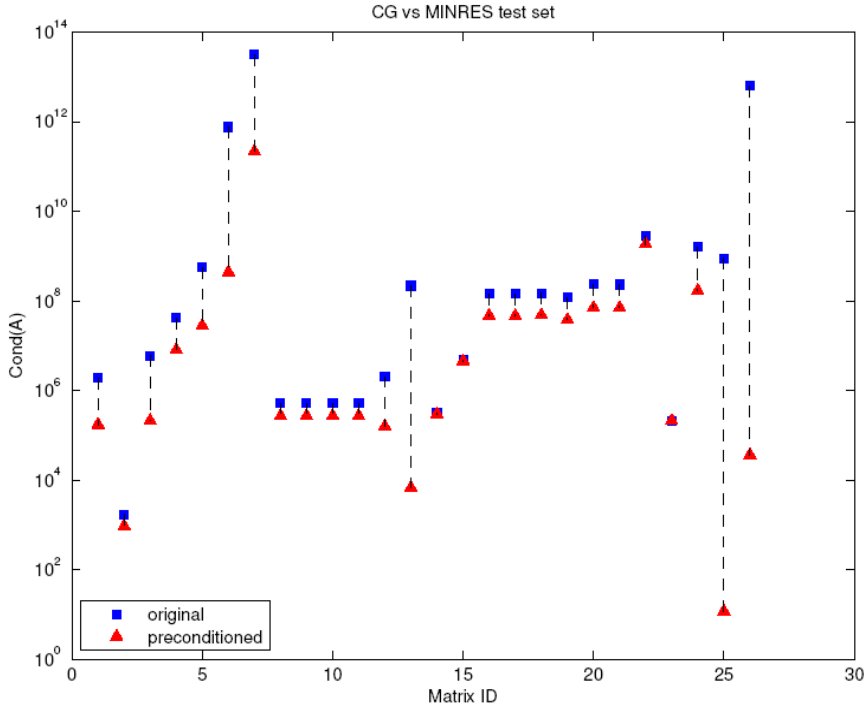
Figure 1. Comparison of distribution of the condition number for matrices used for CG vs MINRES, before and after diagonal preconditioning.
