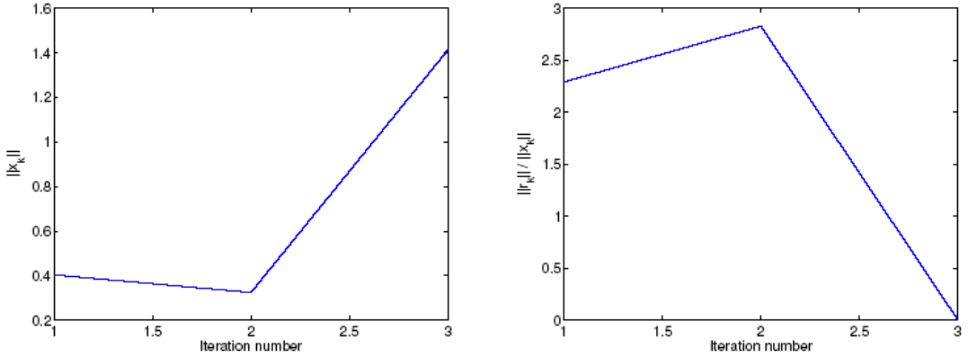
Figure 6. For MINRES on the indefinite problem (4.2), \|x_k\| and the backward error \|r_k\|/\|x_k\| are both slightly non-monotonic.
