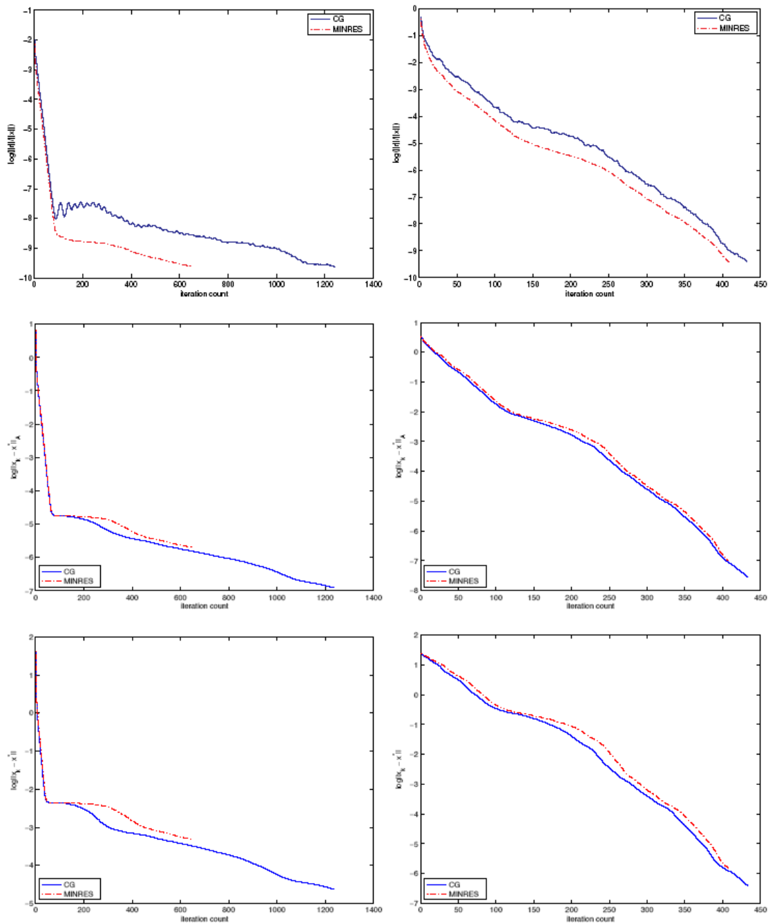
Figure 2. Comparison of backward and forward errors for CG and MINRES solving two spd systems Ax = b .
