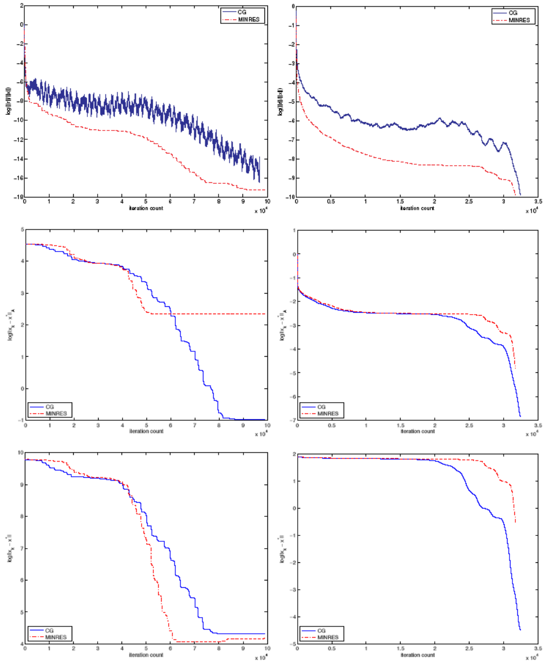
Figure 3. Comparison of backward and forward errors for CG and MINRES solving two more spd systems Ax = b .
