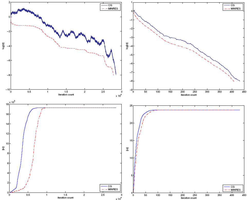
Figure 4. Comparison of residual and solution norms for CG and MINRES solving two spd systems Ax = b .
