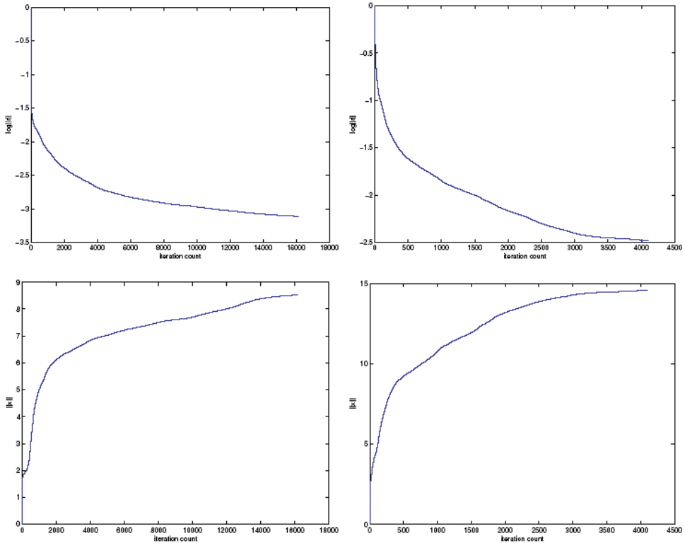
Figure 7. Residual norms and solution norms when MINRES is applied to two indefinite systems (A - \delta I)x = b .
