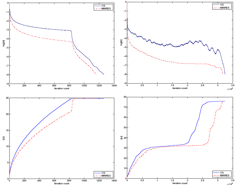
Figure 5. Comparison of residual and solution norms for CG and MINRES solving two more spd systems Ax = b .
