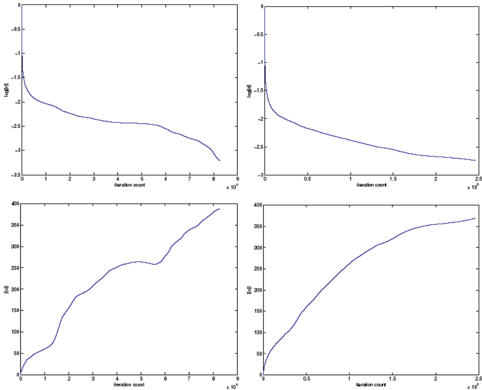
Figure 8. Residual norms and solution norms when MINRES is applied to two more indefinite systems (A - \delta I)x = b .
