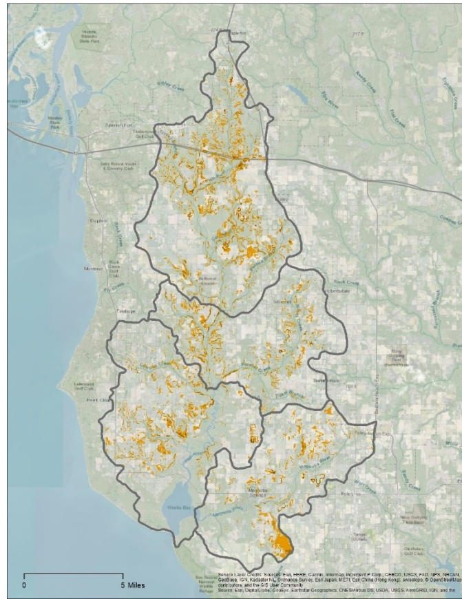
Figure 3.7 High Ranks of Erosion Potential
