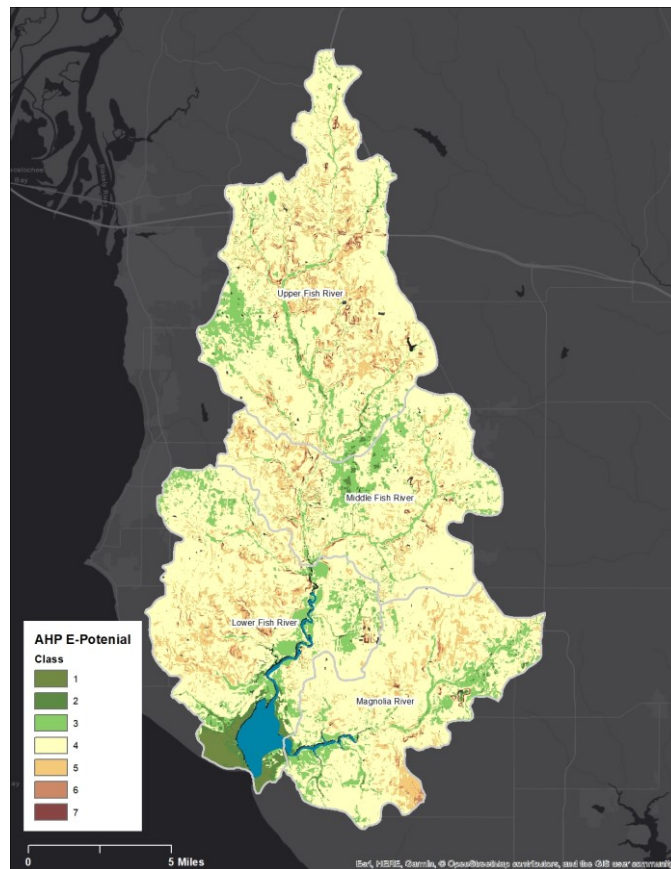
Figure 3.3 Classified AHP Erosion Potential
