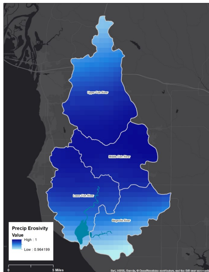
Figure 2.7 Precipitation Erosivity
