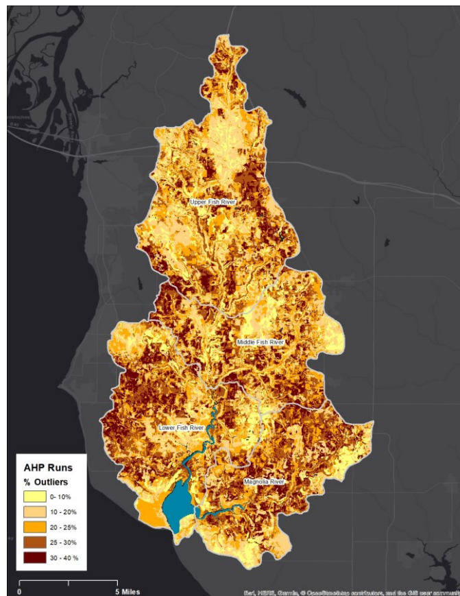
Figure 3.5 Percent Outliers Weighted Data Variations
