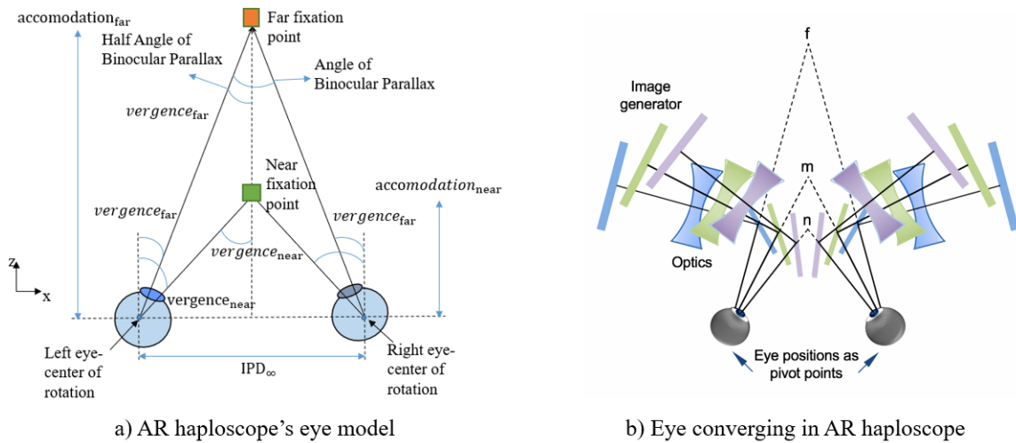
Figure 3.3: a) Eye model of the AR haploscope. b) This figure shows how haploscope's optical system rotates to match with the accurate convergence angle values for different accommodation demand [63].
