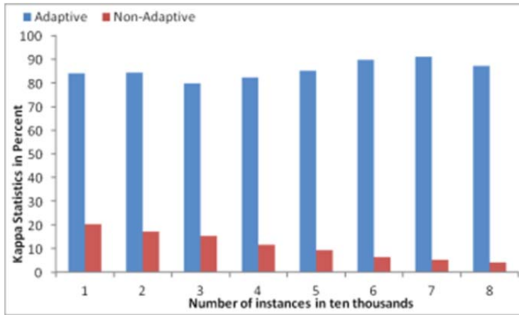
Figure 27 Kappa statistics plot for experiment I
