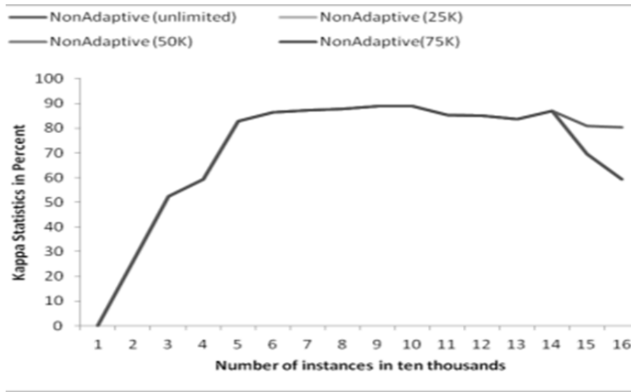
Figure 33 Kappa statistics plot for algorithm with fixed memory
