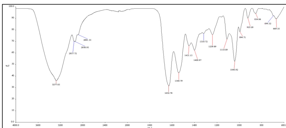
Figure 1: FTIR Spectroscopy of the Film with 1mL CNF Loading
