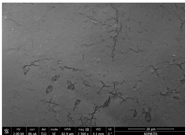
Figure 2. SEM Imaging of the Film with 0.0mL CNF Loading,
