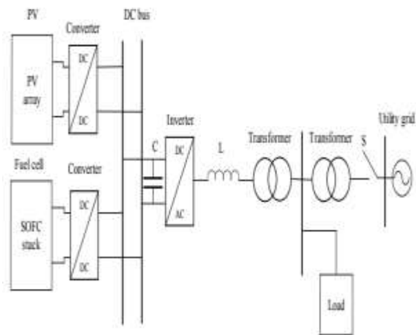
Figure 2 Hybrid solar and fuel cell system
