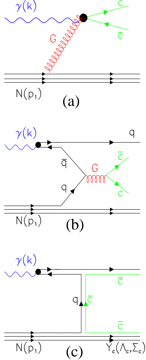
FIG. 2: Feynman diagrams for associative charm production in \gamma N -collisions: (a) the subprocess of photon-gluon fusion \gamma+G \rightarrow c+\bar{c} ; (b) the subprocess of q+\bar{q} -annihilation, q+\bar{q} \rightarrow c+\bar{c} ; (c) t -channel exchange by \bar{D} and \bar{D}^* for \gamma+N \rightarrow Y_c+\bar{D}(\bar{D}^*) .
