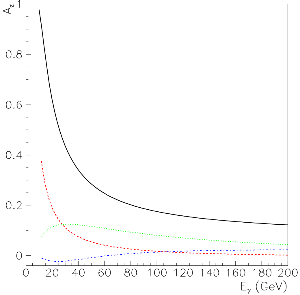
FIG. 13: Integrated \overline{A}_z(E_\gamma) -asymmetry for the reaction \bar{\gamma} + \bar{p} \rightarrow \Lambda_c^+ + \overline{D^0} for ELA approach (solid line), for model I. Predictions for the asymmetry A_{\gamma N}^{c\bar{c}}(E_\gamma) for inclusive charm photoproduction calculated with Eq. 18, taking G(x) and \Delta G(x) from [24] (dashed line), from [26] model B (dotted line), and from [26] model C (dashed-dotted line), are also shown.
