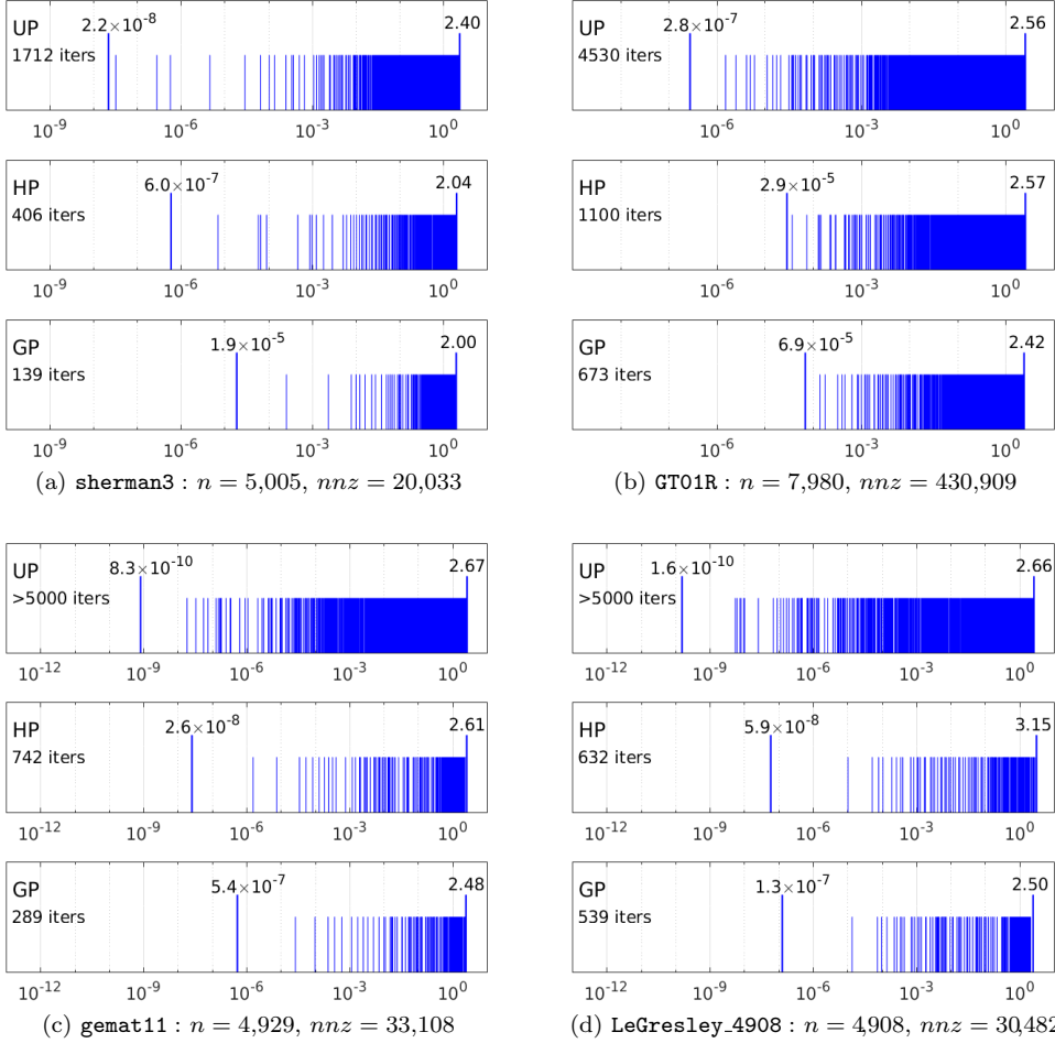
FIG. 8. Eigenvalue spectrum of H (with the smallest and largest eigenvalues) and the number of CG iterations ( iters ) required for convergence.
