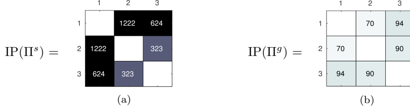
FIG. 5. Inter-block row-inner-product matrix IP(\Pi) for (a) straightforward and (b) “good” block-row partitions.
