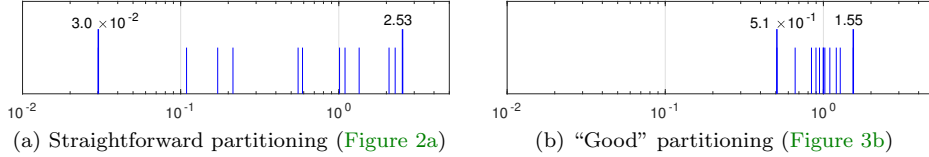
FIG. 6. Eigenvalue spectrum of H for the block-row partitionings of the sample matrix given in Figure 1a.
