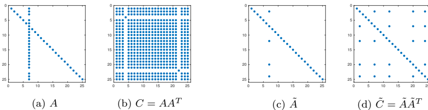
FIG. 7. Nonzero patterns of A , AA^T , \tilde{A} and \tilde{A}\tilde{A}^T .
