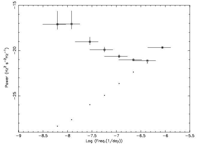
Figure 6. Power density of pulse frequency derivatives of SAX J2103.5+4545, asterisk denotes the instrumental noise.
