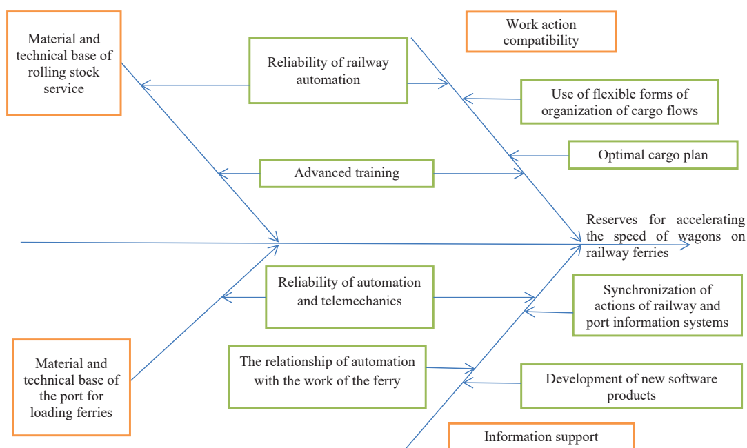
Fig. 1. Ishikawa diagram
