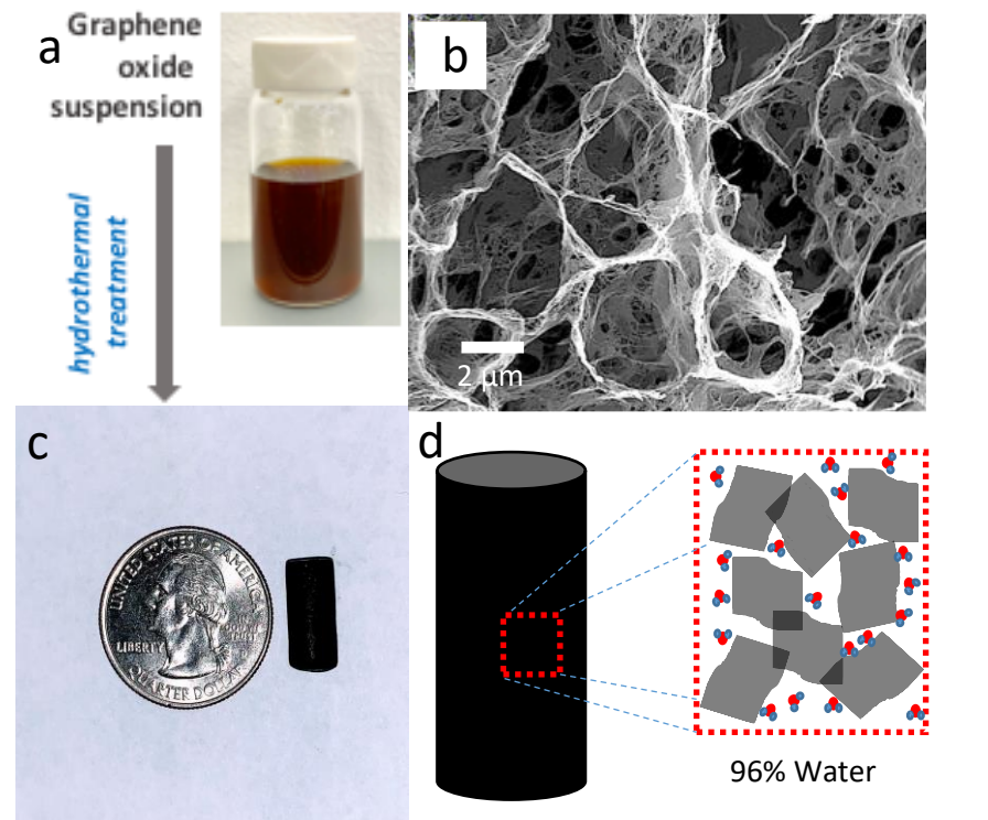
Figure 1: Synthesis and structure of the graphene hydrogel monolith. (a) Graphene oxide nanosheet suspension synthesized by a modified Hummers' method (2 mg/ml stock suspension). (b) SEM image showing a foam-like structure in the interior of the monolith, with micron-sized pores surrounded by thin graphene-based walls. (c) Hydrothermal treatment leads to the porous graphene monolith product shown with scale reference. (d) Sketch showing the hydrophobic sheet-to-sheet interactions leading to gelation and the water association on the remaining oxygen-containing surfaces.
