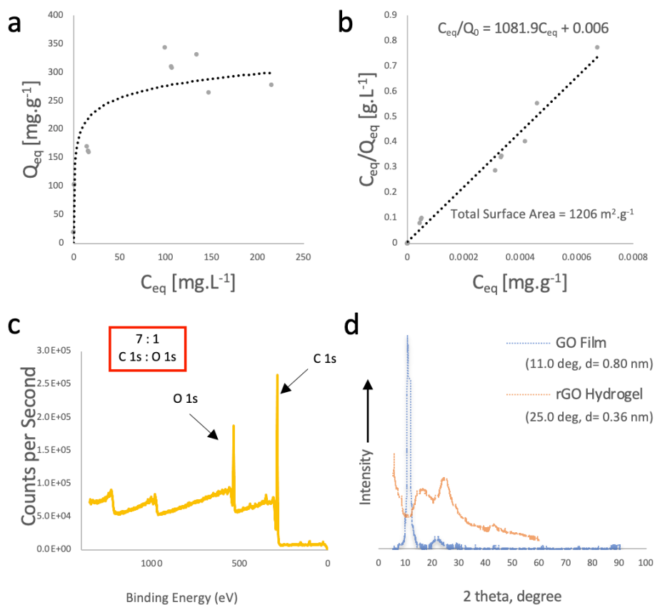
Figure 2: a) Methylene blue adsorption isotherm used for surface area determination; b) Linearization and fit to Langmuir isotherm. c) XPS spectra showed a change in the carbon oxygen ratio from ~2:1 (original GO precursor [see SI]) to ~7:1 in the hydrothermally treated monolith. d) XRD analysis also shows a change in the interlayer spacing from 0.80 nm (GO) to 0.36 nm (rGO-HG) which reflects the loss of oxygen functional groups between individual sheets.
