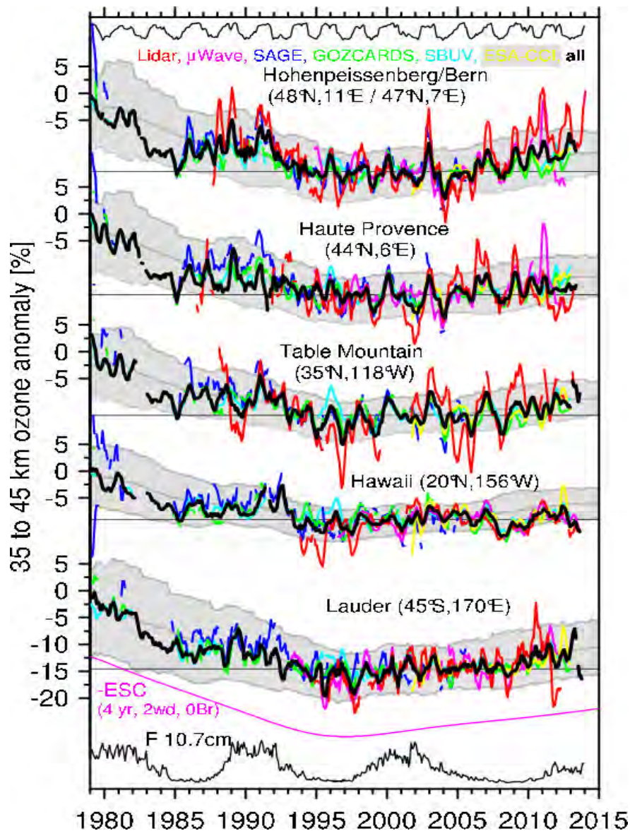
Figure 1.3 Time series of ozone anomalies in the upper stratosphere as observed by ground-based lidars and microwave radiometers at five stations of the Network for the Detection of Atmospheric Composition Change (NDACC) and by satellite instruments. Anomalies are derived by subtracting the average annual cycle of each data record between 1998 and 2008, but the percent scale is set to zero at the beginning of data in 1979. Satellite data are 10° zonal means centred at the station latitudes. The GOZCARDS data record merges SAGE and HALOE data (up to 2005) with AURA-MLS data (since 2004) (Froidevaux et al., 2014). SBUV is the SBUV V8.6 merged dataset provided by NASA (McPeters et al., 2013). ESA-CCI is the average anomaly from the OSIRIS and SMR datasets (since late 2000), and the GOMOS, MIPAS, and SCIAMACHY satellite datasets (2002 to spring 2012) and was processed under the ESA Climate Change Initiative (Sofieva et al., 2013). The thick black line is the average anomaly from all available data sets. For clarity, data are smoothed by a 5 month running mean. The grey underlay is obtained from CCMVal-1 model simulations. It gives the running 24 month multi-model mean and \pm 2 standard deviations of individual model monthly means from this mean. The black lines at the top and bottom give proxies for QBO and solar flux. The pink line at the bottom gives an (inverted) proxy for stratospheric chlorine loading. Weber et al., 2014, updated from Steinbrecht et al. 2009.
