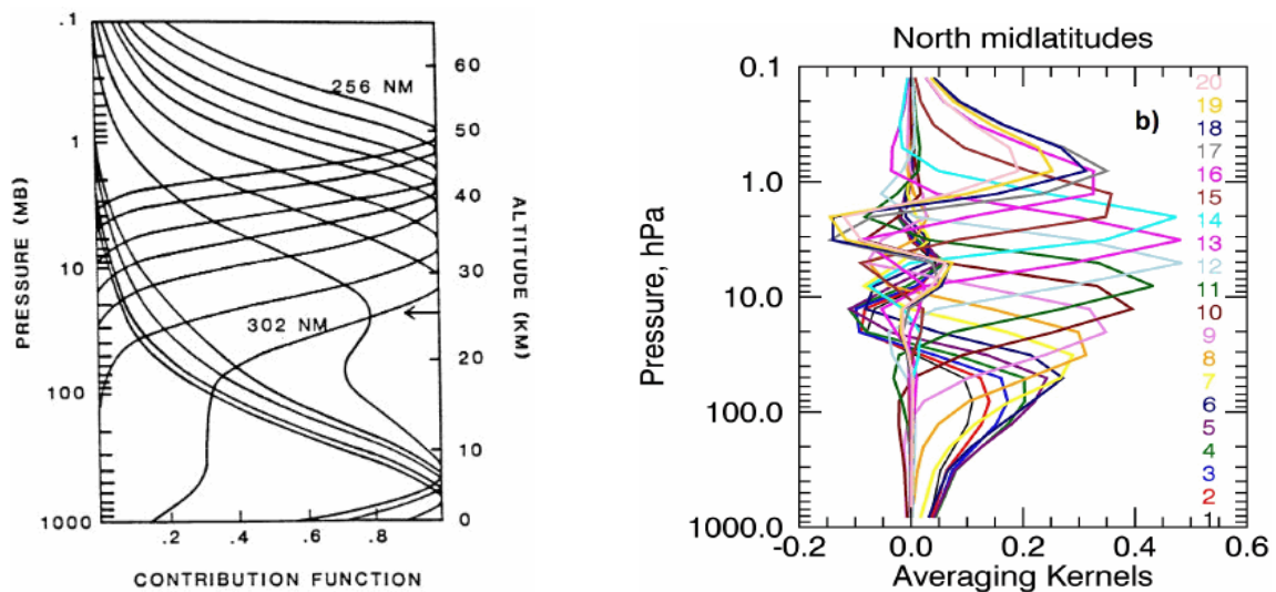
Figure 3.2 Contribution functions (left, Fleig et al., 1990) and averaging kernels (right, Kramarova et al., 2013) typical for SBUV nadir ozone profile retrievals. Twelve discrete wavelengths between about 255 nm and 340 nm are used in the SBUV-type retrieval (Barthia et al., 2013). The wavelengths below about 300 nm contain profile information (upper curves in left panel), while the longer wavelengths (lower curves) provide total ozone information. The averaging kernels (right panel) for altitudes below the ozone number density peak ( \sim 22 km, \sim 40 hPa) are getting broader (lower vertical resolution) and more asymmetric (larger smoothing errors).
