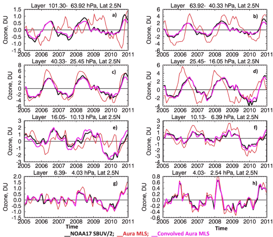
Figure 3.4 Monthly mean zonal mean de-seasonalised ozone (anomaly) timeseries from SBUV2 and MLS/Aura (limb) for different altitudes in the inner tropics. Note the change in the phase and amplitude of the SBUV2 QBO signal due to the averaging kernels in the lower stratosphere. From Kramarova et al. (2013b).
