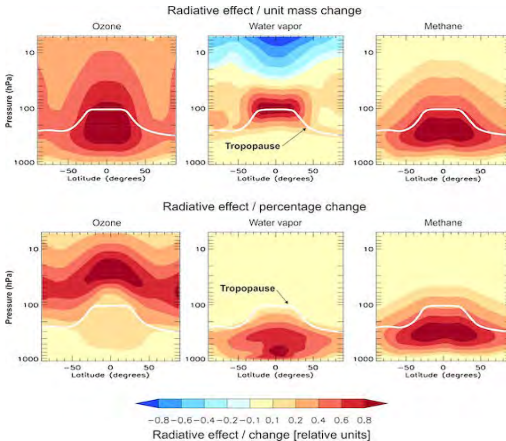
Figure 1.7 Sensitivity of surface temperature to the altitude and latitude of (left) ozone, (middle) water vapour, and (right) methane changes. Shading shows relative impact on surface temperature, measured as radiative effect, from either (top) unit mass increases or (bottom) 1% increases applied at individual latitudes and altitudes (1 km thick layers). For each trace gas, the calculated radiative effects have been normalized to the respective maximum value. Red colours are indicative of warming, blue colours indicate cooling. (Figure taken from Riese et al. (2012)).
