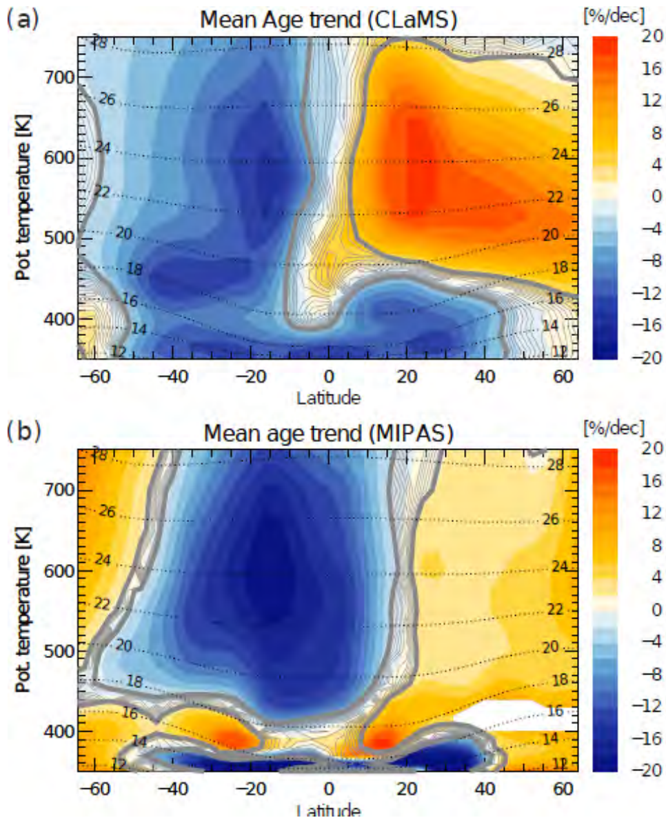
Figure 1.4 Relative linear trend (in percent) of zonal mean age of air for the period 2002-2010 from (a) CLaMS and (b) MIPAS. The significance of the trend, measured in multiples of the standard deviation ( \sigma ), is shown as grey contours ( 2\sigma contour as thick lines, then decreasing with 0.2 steps as thin lines). Dashed lines show altitude levels in km. (From Ploeger et al., 2015).
