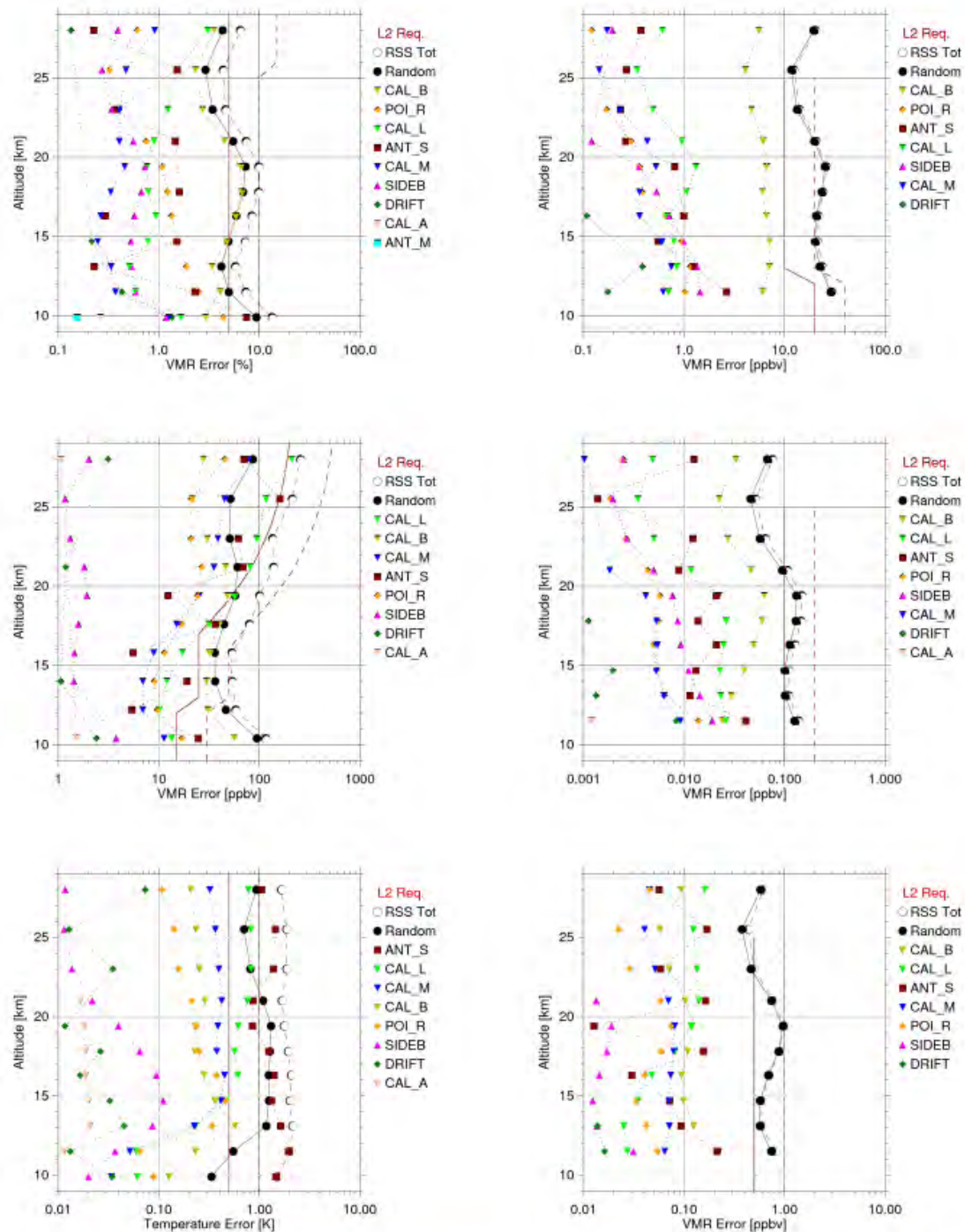
Figure 3.7 From the PREMIER study (CORSA study final report) – Summary plots for H 2 O (top left), CO (top right), O 3 (centre left), HCN (centre right), T (bottom left), HNO 3 (bottom right) based on STEAM-R Level 1 performance estimates for the industrial phase-A study. Error budgets calculated by J. Urban are according to Level-1 instrument performance estimates reported in the report for mission selection and a standard retrieval set-up for linear simulations. Only instrumental errors are considered, spectroscopic errors are not included.
