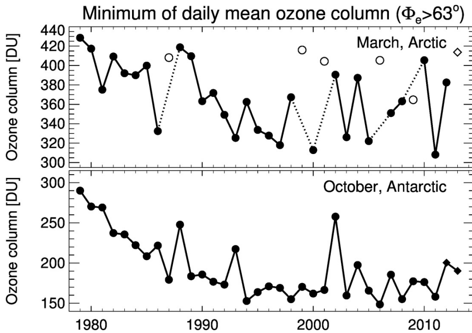
Figure 1.2 Time series of the minimum of the daily average column ozone (Dobson units) within the 63^\circ contour of equivalent latitude ( \Phi_e ) in March in the Arctic and October in the Antarctic. Arctic winters in which the polar vortex broke up before March (1987, 1999, 2001, 2006, 2009, and 2013) are shown by open symbols; dotted lines connect surrounding years. Figure adapted and updated from Müller et al. (2008) and WMO (2014), using the Bodeker Scientific combined total column ozone database (version 2.8; circles) through the Arctic winter of 2012, and Aura OMI measurements thereafter (diamonds). (Figure courtesy of Jens-Uwe Grooß).
