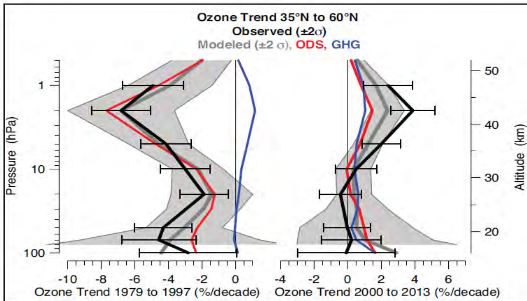
Figure 1.1 Vertical profiles of observed annual mean ozone trends over 35°N–60°N (black) for the periods of stratospheric ODS increase (left) and ODS decline (right), with the corresponding trends based on model simulations (CCMVal-2) for ODS changes only (red), GHG changes only (blue), and both together (grey). The \pm 2 standard error uncertainty range for the trends is shown by the horizontal bars for the observations and by the grey shading for the all-changes modelled trend. (From WMO, 2014).
