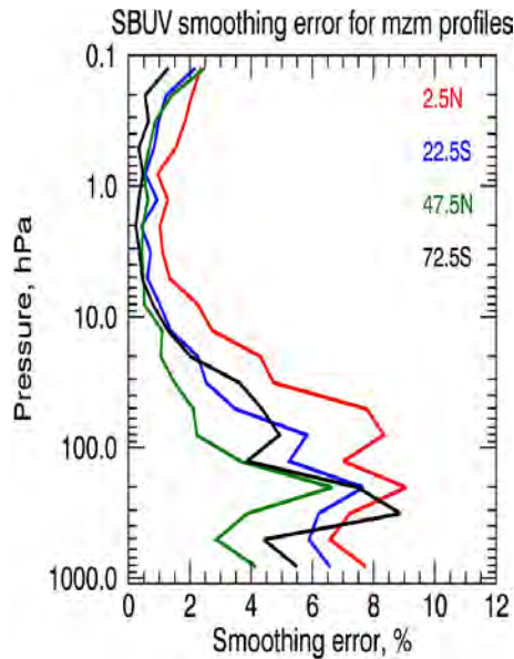
Figure 3.3 Smoothing errors of monthly mean zonal mean (mzm) ozone. From Kramarova et al. (2013a).
