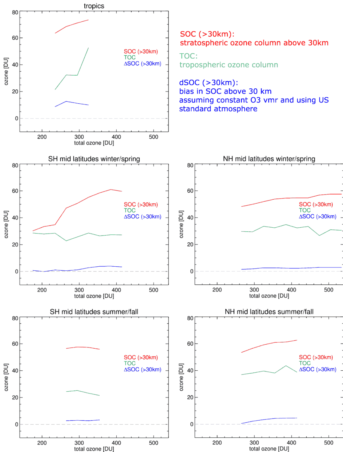
Figure AB.2 Stratospheric ozone columns (SOC) and tropospheric ozone columns (TOC) as derived from the Lamsal et al. (2004) ozone profile climatology (Fig. BOX1). Top panel: tropics; middle panel: middle latitudes in the SH (left) and NH (right) in winter/spring; bottom panels: same as the middle panels but for summer/fall.
