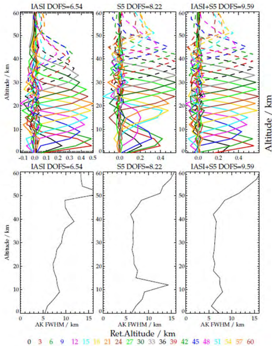
Figure 3.1 Theoretical averaging kernels for left: the next generation IASI instrument on METOP-SG (thermal infrared), Sentinel 5 (UV/visible) and the combination of the two. Simulations have been performed assuming 100% a priori error and a correlation length of 3km only; this is a looser constraint than would be applied in reality but allows the theoretical information that could be provided by the instrument to be assessed. The bottom row of plots shows the achievable vertical resolution, represented by the full width half maximum of the averaging kernels.
