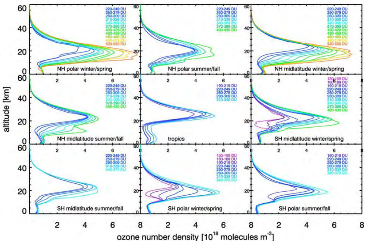
Figure AB.1 Climatological ozone profiles from Lamsal et al. (2004).
