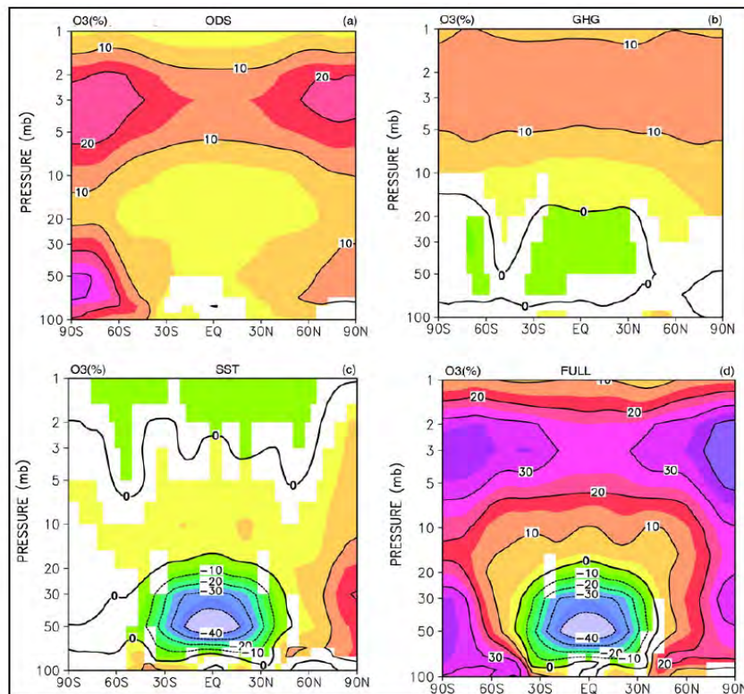
Figure 1.6 Zonal, annual and ensemble mean percentage changes of the ozone mixing ratio between different timeslice integrations of the SOCOL CCM for 2100 and for 2000 conditions. (a) Ozone changes from 2000 to 2100 when only ODSs are changed. (b) Ozone changes from 2000 to 2100 due to GHG changes only. (c) Ozone changes due to changes in sea surface temperature and sea ice, driven by tropospheric warming. (d) Ozone changes when ODS, GHG, sea surface temperature, and sea ice are all changed together. White regions indicate non-significant changes at the 5% confidence level. Adapted from Zubov et al. (2013) and WMO (2014).
