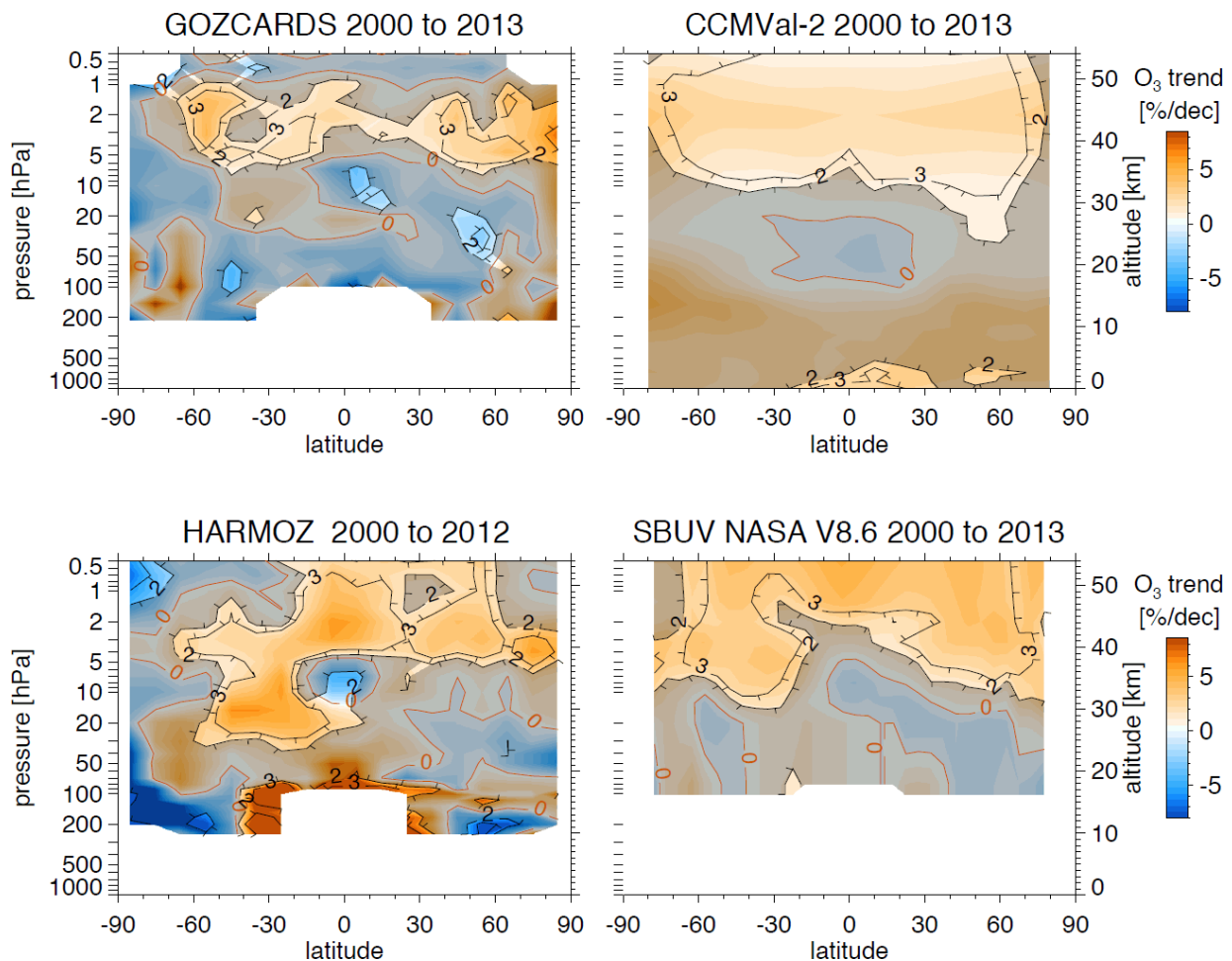
Figure 3.5 Ozone profile trends in %/decade after 2000 from different profile datasets. Left top: GOZCARDS limb data (merged SAGE II and MLS/Aura data), top right: CCMVal-2 dataset combining several chemistry climate models (CCM), bottom left: HARMOZ (merged ENVISAT and ODIN limb data), bottom right: SBUV V8 nadir profile data. Magnitudes of trends are given by the colour scale. The black contour lines give the ratio of trend to uncertainty, i.e., the statistical significance of the trends. The line labelled 3 corresponds to 3\sigma , 2 corresponds to 2\sigma . Gray shading indicates regions where the trends are not significant at the 2\sigma level. (WMO, 2014).
