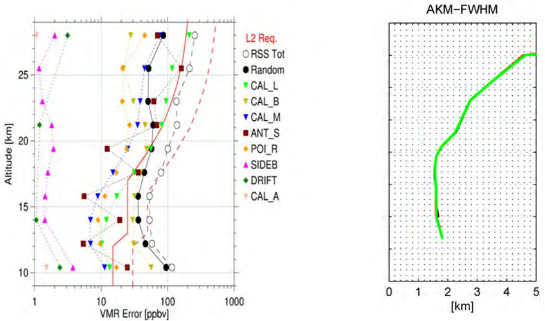
Figure 3.6 STEAM-R simulations of uncertainties and vertical resolution for an instrument measuring at tangent altitudes from 6 to 28 km (in the context of the study for the PREMIER mission). In subsequent studies the limb-viewing range has been extended to include the whole stratosphere leading to compliance with the minimum mission ‘Operoz’ requirements over the full required altitude range.
